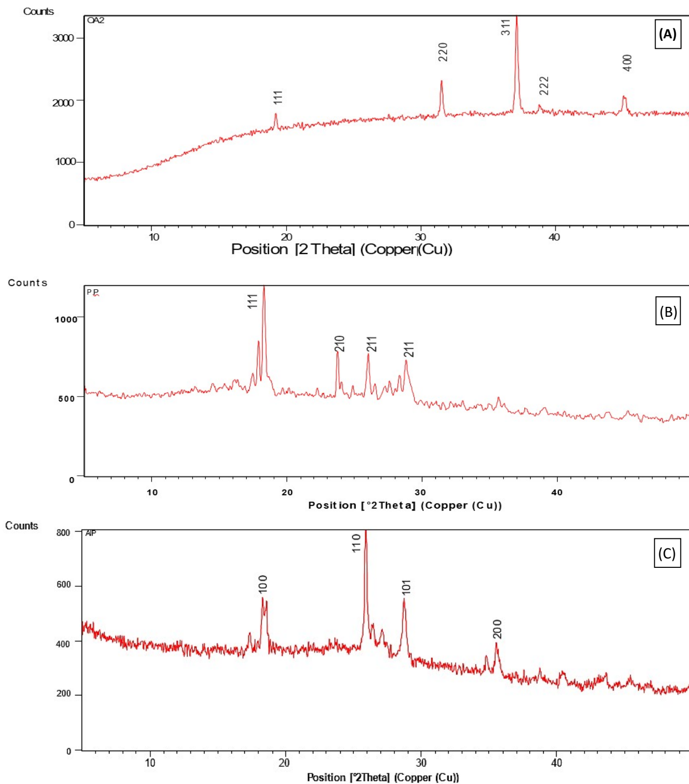
Fig. S4. Powder XRD of Co 3 O 4 QDs (A), PPy (B), and Co 3 O 4 @PPy NCs (C).
