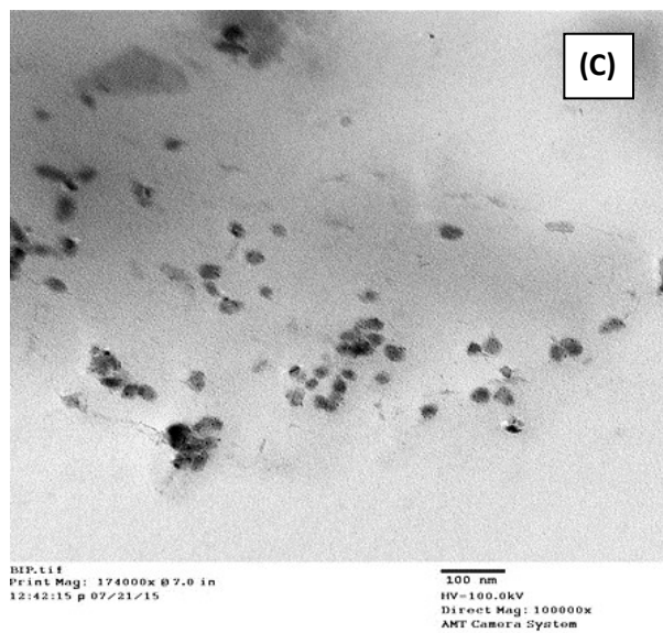
Fig. S5 (ESI). TEM images of Co 3 O 4 QDs (A), PPy CPs (B), and Co 3 O 4 @PPy NCs (C and D).
