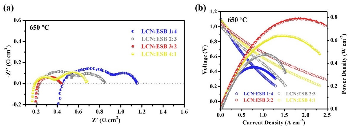
Figure. S1 Electrochemical performance of single cells after 2 h polarization: (a) EIS curves, (b) I-V-P curves.
