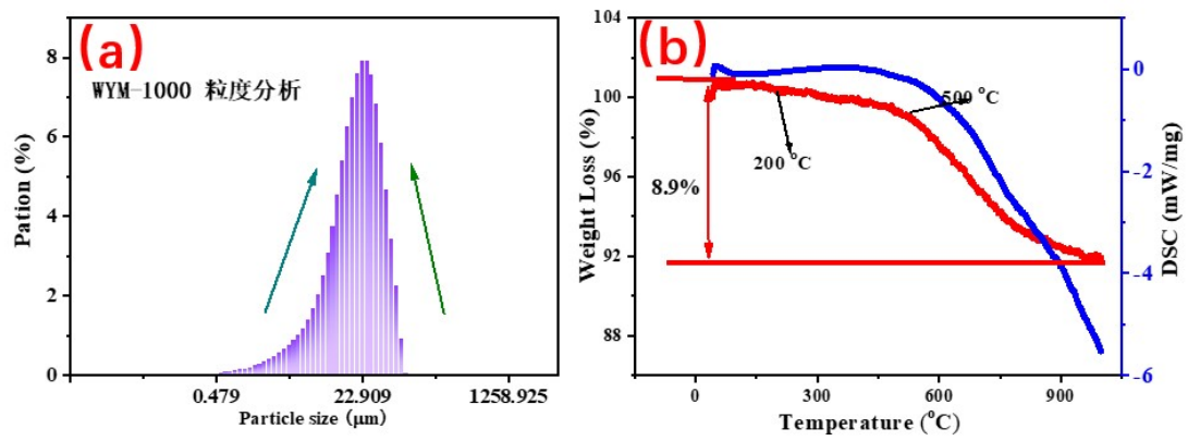
Fig.S1 For WYM-1000 samples, the particle size distribution, and TG curves
