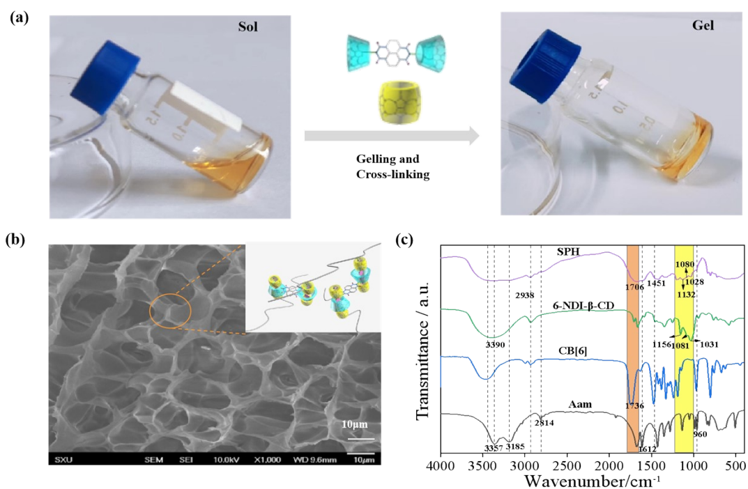
Fig. 3 (a) A mixture of water, Paxle, 6-NDI-β-CD, and CB[6] in a 62:19:4:15 ratio before (left) and after heating at 70°C for 30 min and cooled down to room temperature (right). (b) SEM image and (c) FTIR spectrums of SPH.
