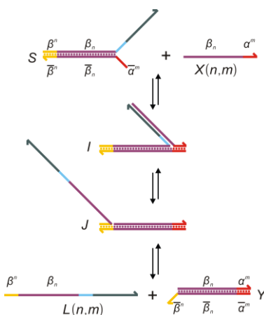
Fig. 1S The detailed illustration of the formation process as correct Catassembler is introduced.
