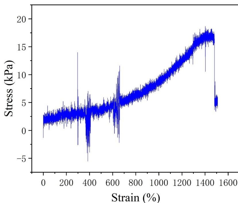
Figure S1. Stress-strain curve of the cut sample after self-healing treatment via contacting the cut parts for 30 min at ambient temperature.
