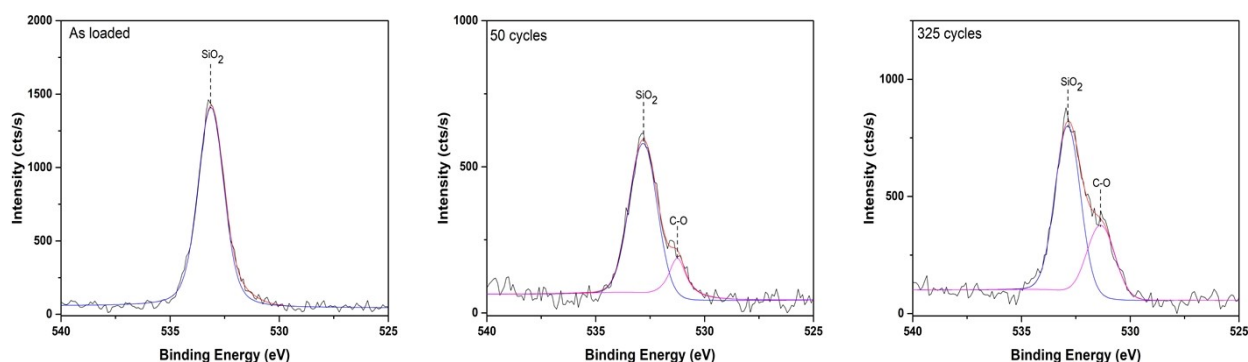
Figure S3 O1s high resolution spectra of 40K 1.5wt% as loaded, 50 and 325 cycles into the ALD process.
