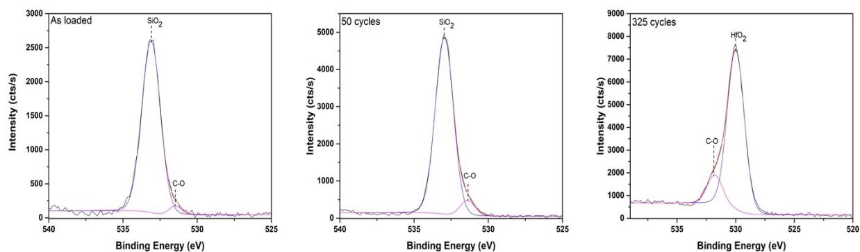
Figure S1 O1s high resolution spectra of 16K 1.5wt% as loaded, 50 and 325 cycles into the ALD process.
