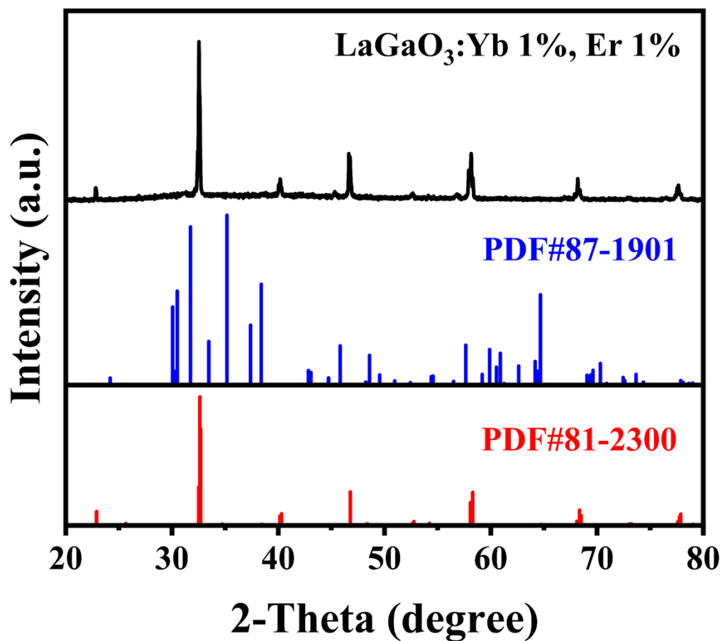
Figure S1. The XRD patterns of LaGaO 3 :1% Yb, 1% Er and standard pattern (PDF# 81-2300 LaGaO 3 ) and (PDF# 87-1901 Ga 2 O 3 ).
