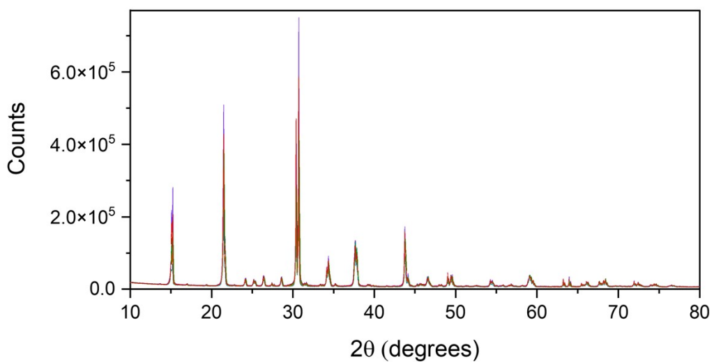
Figure S2. Powder XRD plot of a series of parallel crystal. The peak positions are consistent with an orthorhombic crystal structure.
