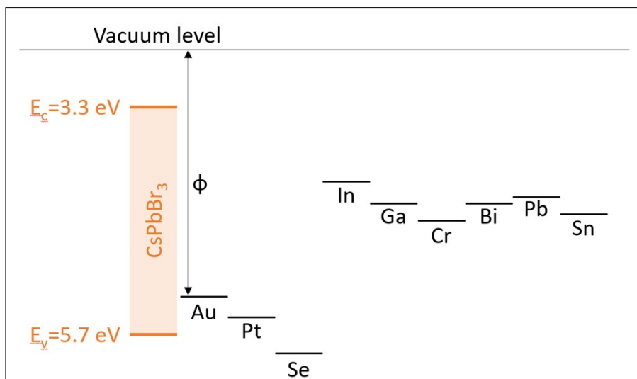
Figure S1. Energy band diagram of CsPbBr 3 and work function of different metal contacts.
