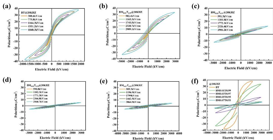
Fig. S1 Changes of electrical hysteresis loop of BM x T(1-x) films.
