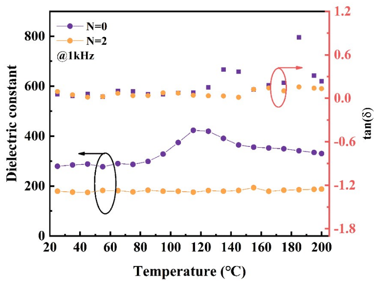
Fig. S2 Temperature dependences of dielectric property for N=0 and N=2.
