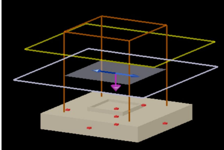
Fig. S1. Schematic of the FDTD calculation for the metal residue.
