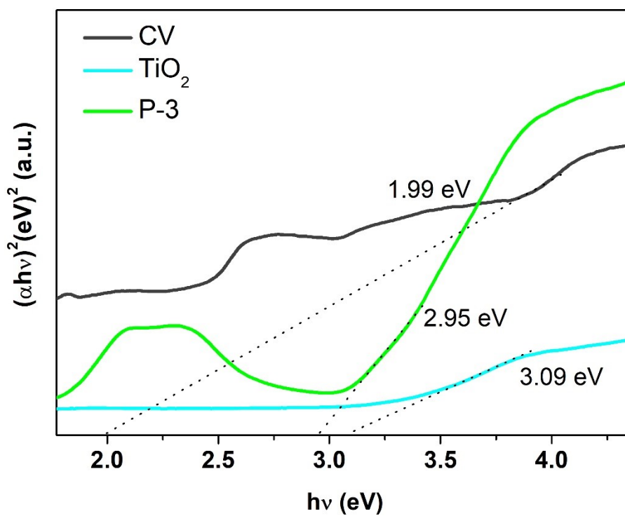
Figure S1. The converted Tauc plot of (\alpha h\nu)_2 versus photon energy ( h\nu ) of CV, \text{TiO}_2 and P-3 photocatalysts.
