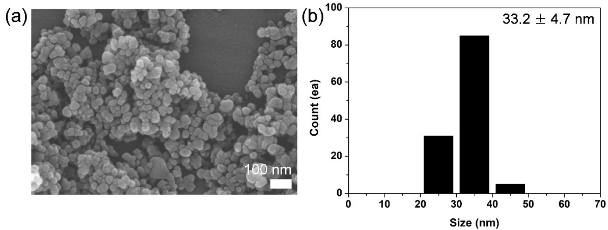
Figure S2. (a) SEM image and (b) the corresponding size-distributions of the P-3 photocatalyst.
