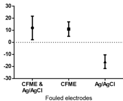
(c) Peak oxidative voltage shift (mV)
