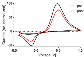
CFME fouled (normalized)
