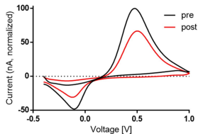
CFME and Ag/AgCl electrode fouled (normalized)
