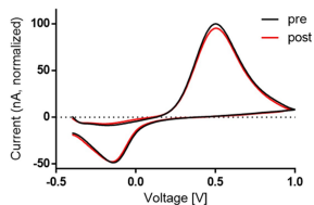
Ag/AgCl fouled(normalized)
