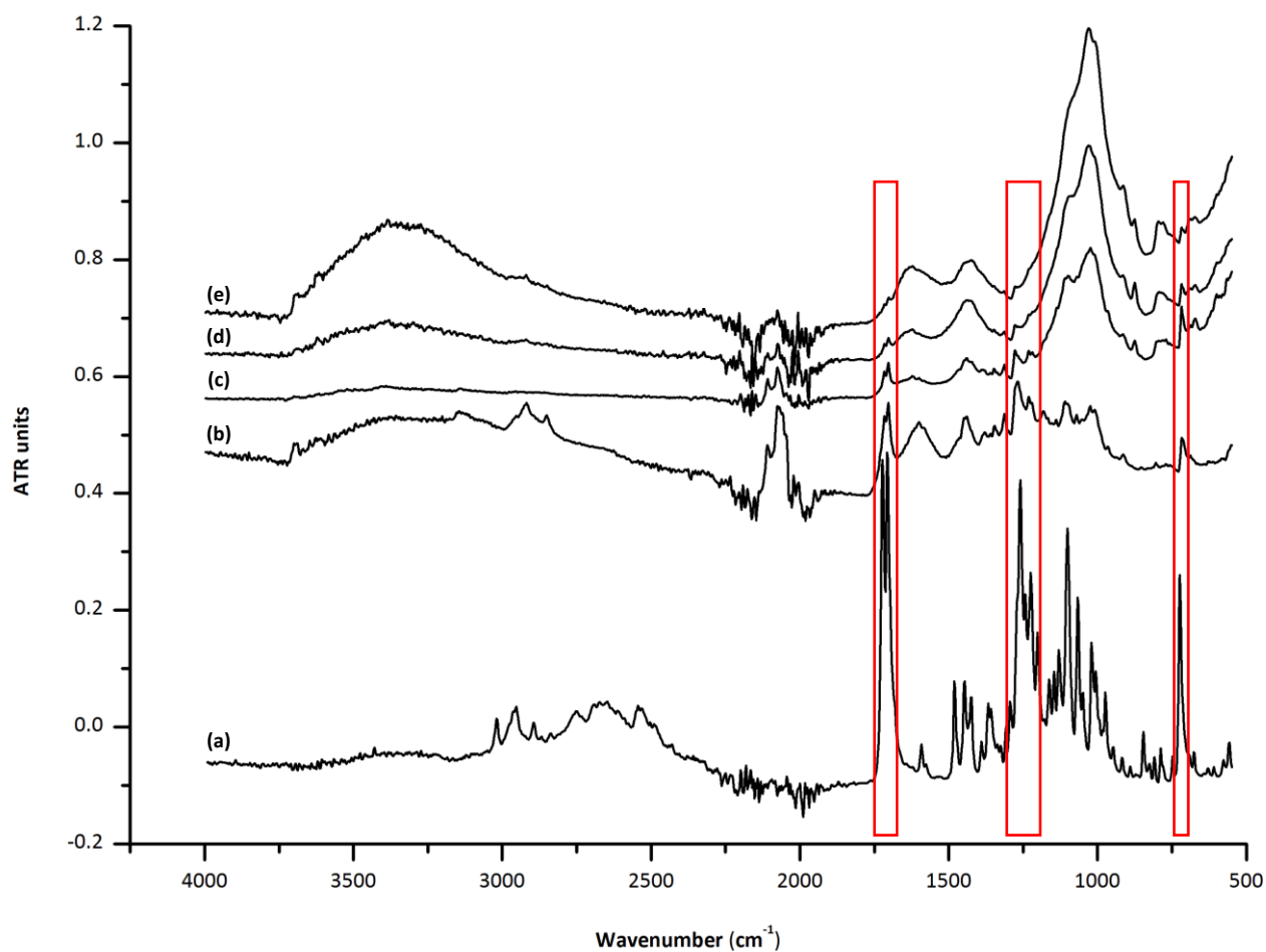
22 Figure S1. Direct ATR-FTIR spectra of cocaine hydrochloride standard (a) and powdered carbon (b), soil 23 (c), coconut fiber (d) and ground palm kernel shell (e) seized camouflaged samples positive in cocaine. 24 Note: The main characteristic bands of cocaine are indicated by the boxes.
