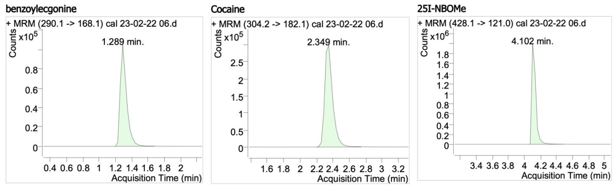
Fig. S2. Chromatograms of the nine target compounds (50 µg/L).
