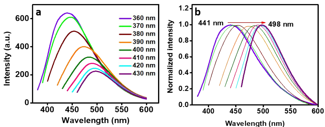
Figure S1 a) Excitation wavelength dependent emission spectra of LL-CDs , b) Normalized spectra
