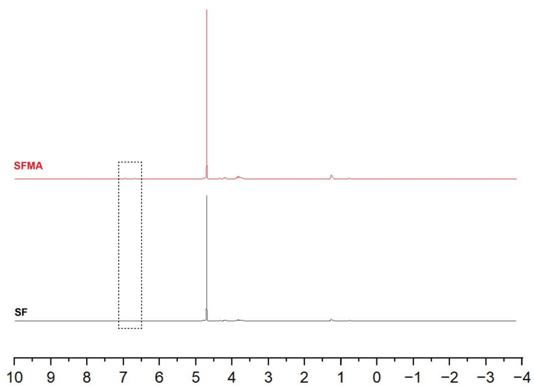
Fig. s1 1 H-NMR spectra of SF and SFMA.
