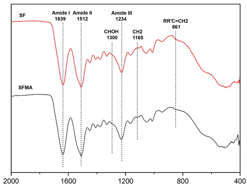
Fig. s2 FTIR spectra of SF and SFMA
