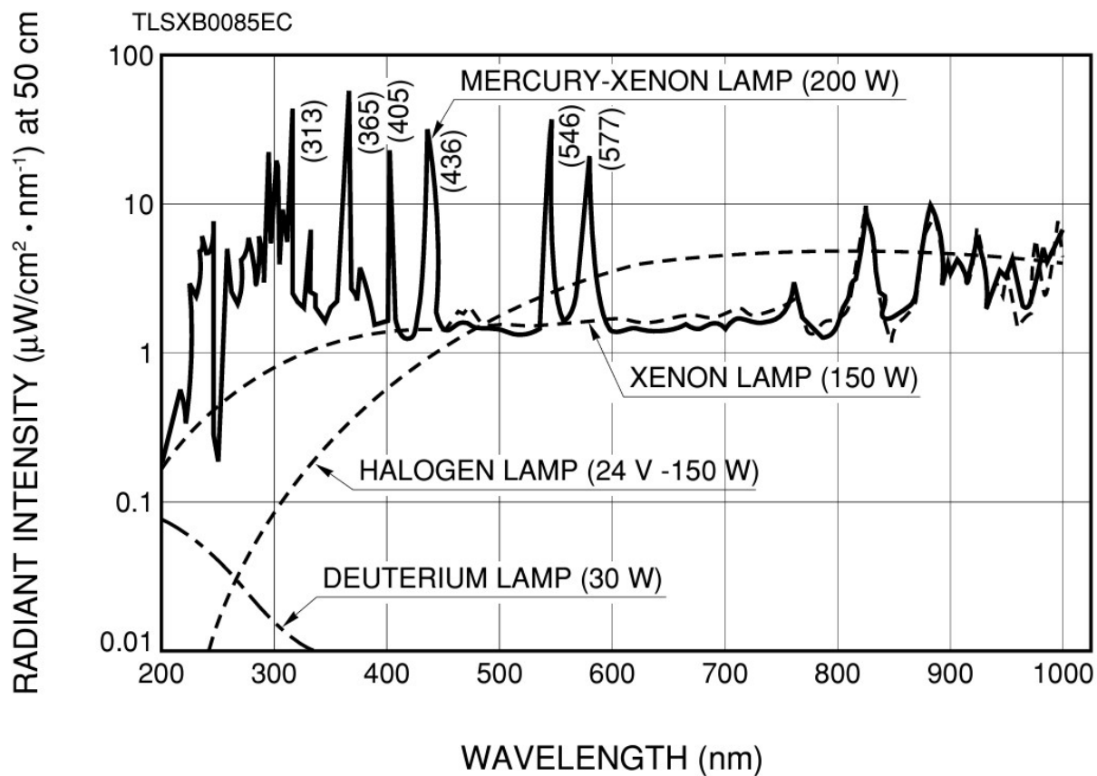
Figure S1: The radiation spectrum of the Hamamatsu L2570 200 W HgXe arc lamp with comparison to deuterium, halogen and xenon lamps. Reproduced from manufacturer's specification.
