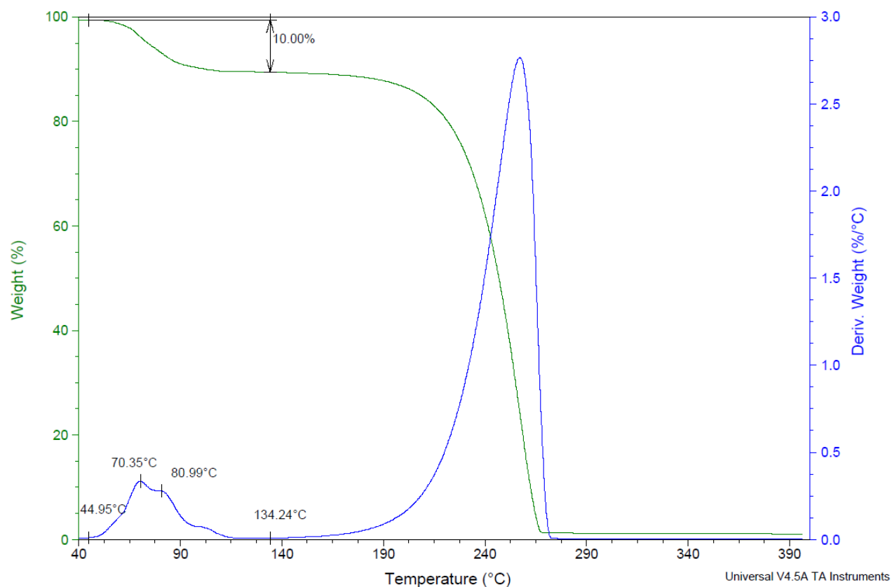
Fig S1. Overlaid TG and DTG traces for a) 2(H1)·PYR, b) 2(H1)·2MP, c) 2(H1)·3MP and d) 3(H1)·4MP.
