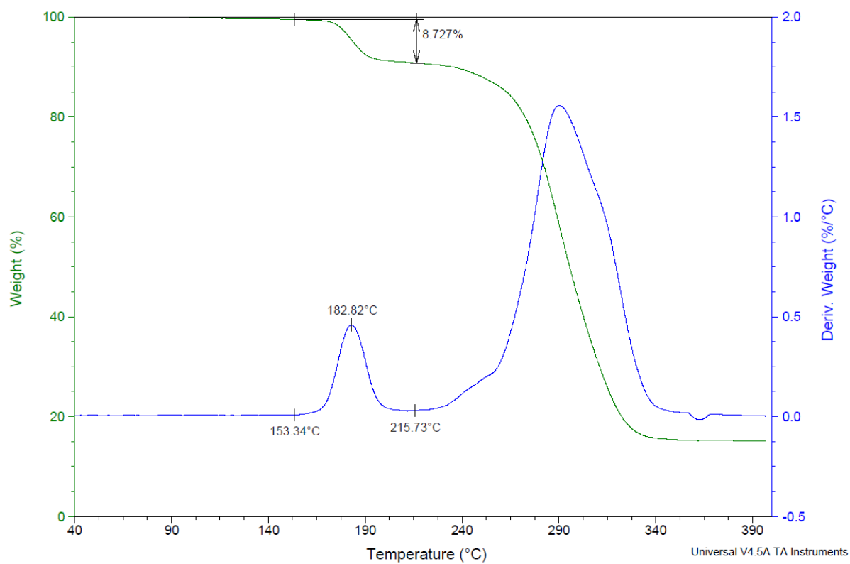
Fig S3. Overlaid TG and DTG traces for a) H3-PYR, b) H3-2MP, c) H3-3MP and d) H3-4MP.
