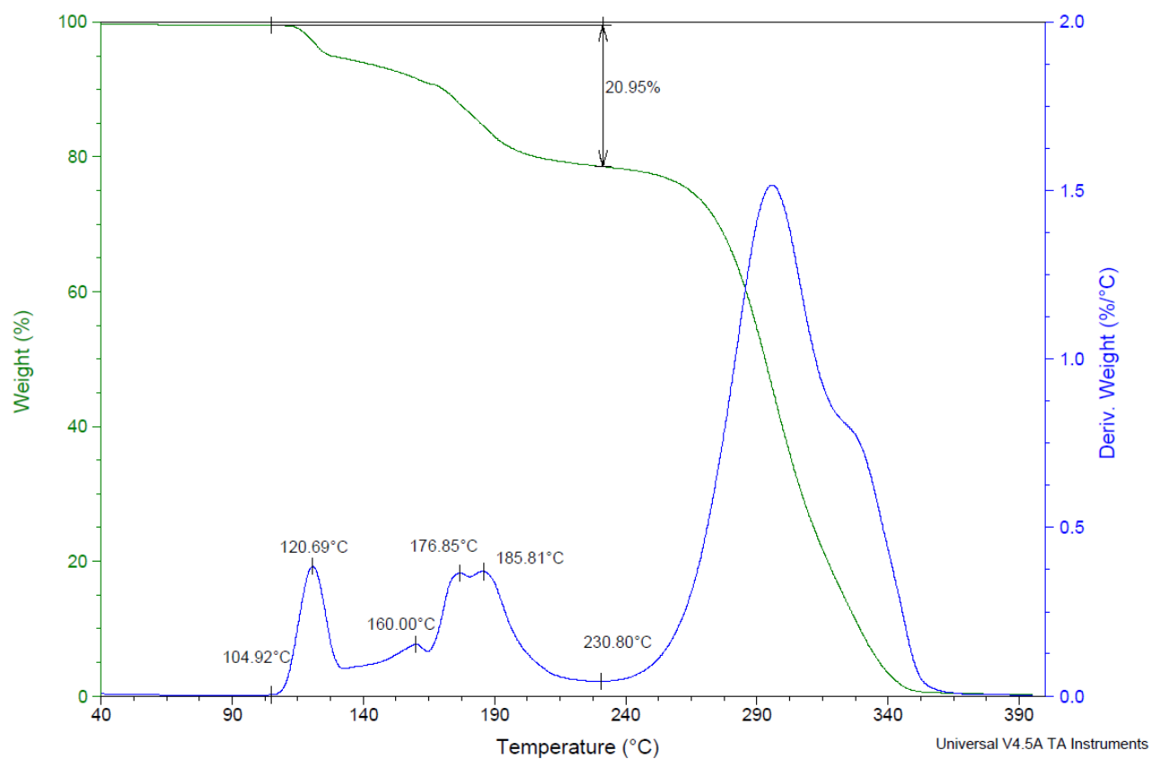
Fig S2. Overlaid TG and DTG traces for a) 2(H2):3(PYR), b) H2-2MP and c) 2(H2):3(3MP).
