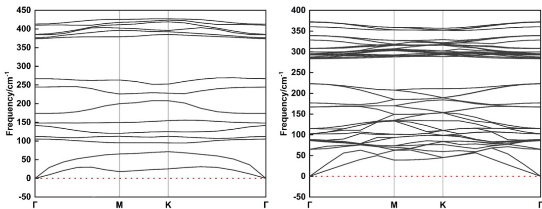
Figure S1 (a) phonon spectrum of AlAs monolayer, (b) phonon spectrum of GaS monolayer.
