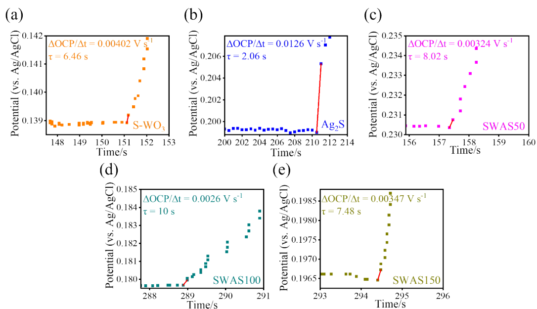
Fig. S2 The carrier lifetime of various samples derived from OCP decay curves at the transient when illumination is removed; (a) S-WO 3 , (b) Ag 2 S, (c) SWAS50, (d) SWAS100, and (e) SWAS150.
