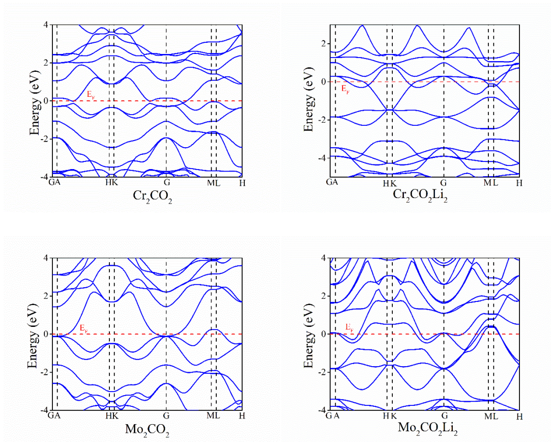
Fig. S3. Band structures of different MXenes before and after lithiation.
