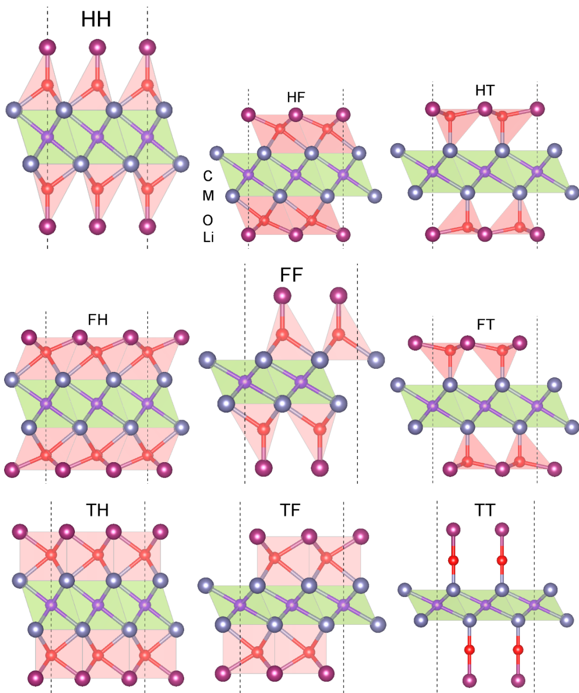
Fig. S1. Nine constructed lithiated XY-M_2CO_2Li_2 configurations
