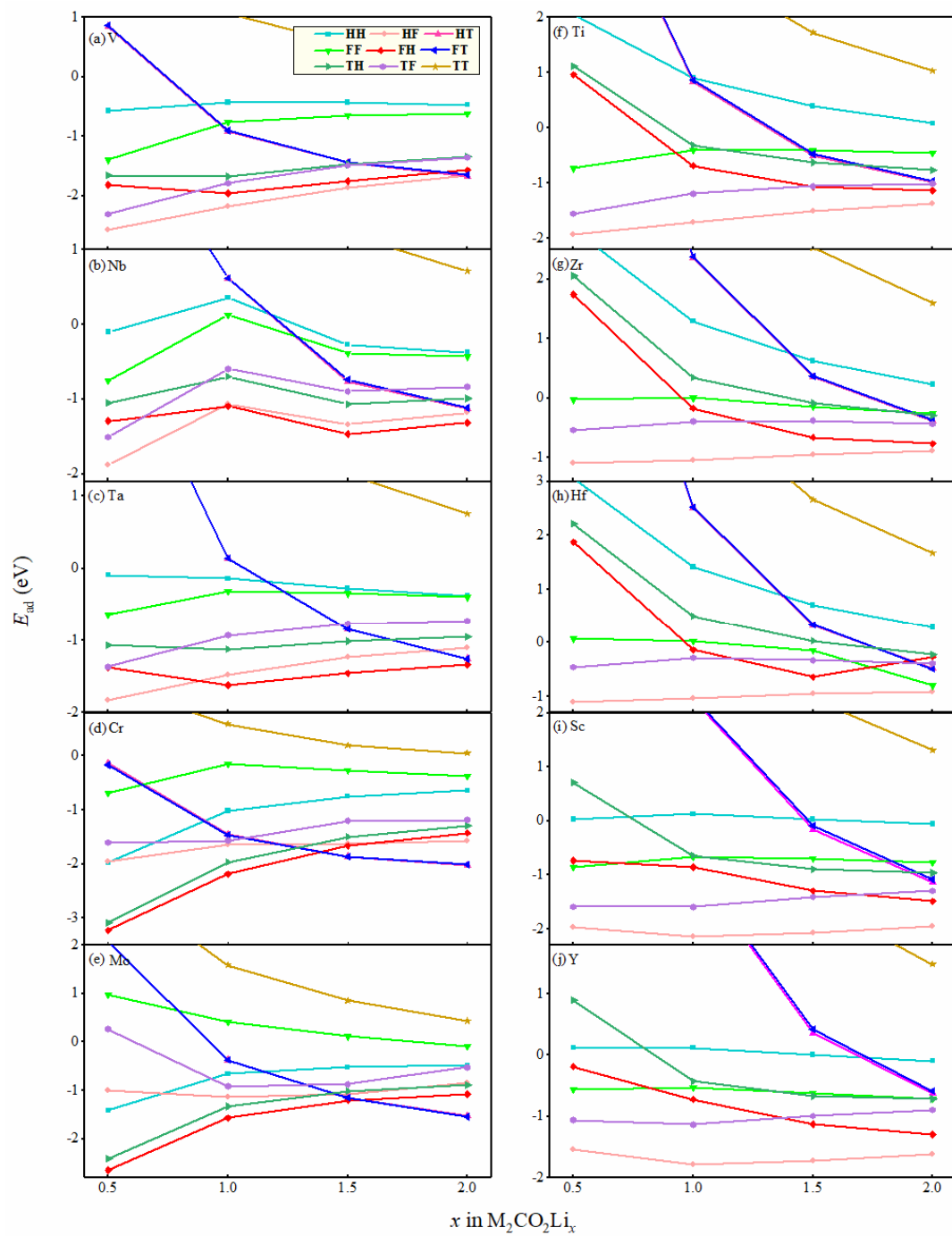
Fig. S2. Adsorption energies of different M_2CO_2Li_x configurations with a variable of Li contents ( x values)
