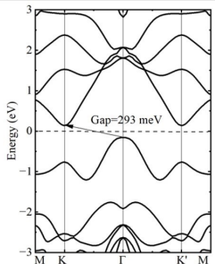
(a) CrSiGeN 4
