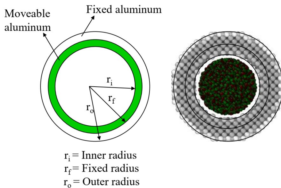
Figure S1 Design of an aluminum nanotube using reactive molecular dynamics simulations of water splitting.
