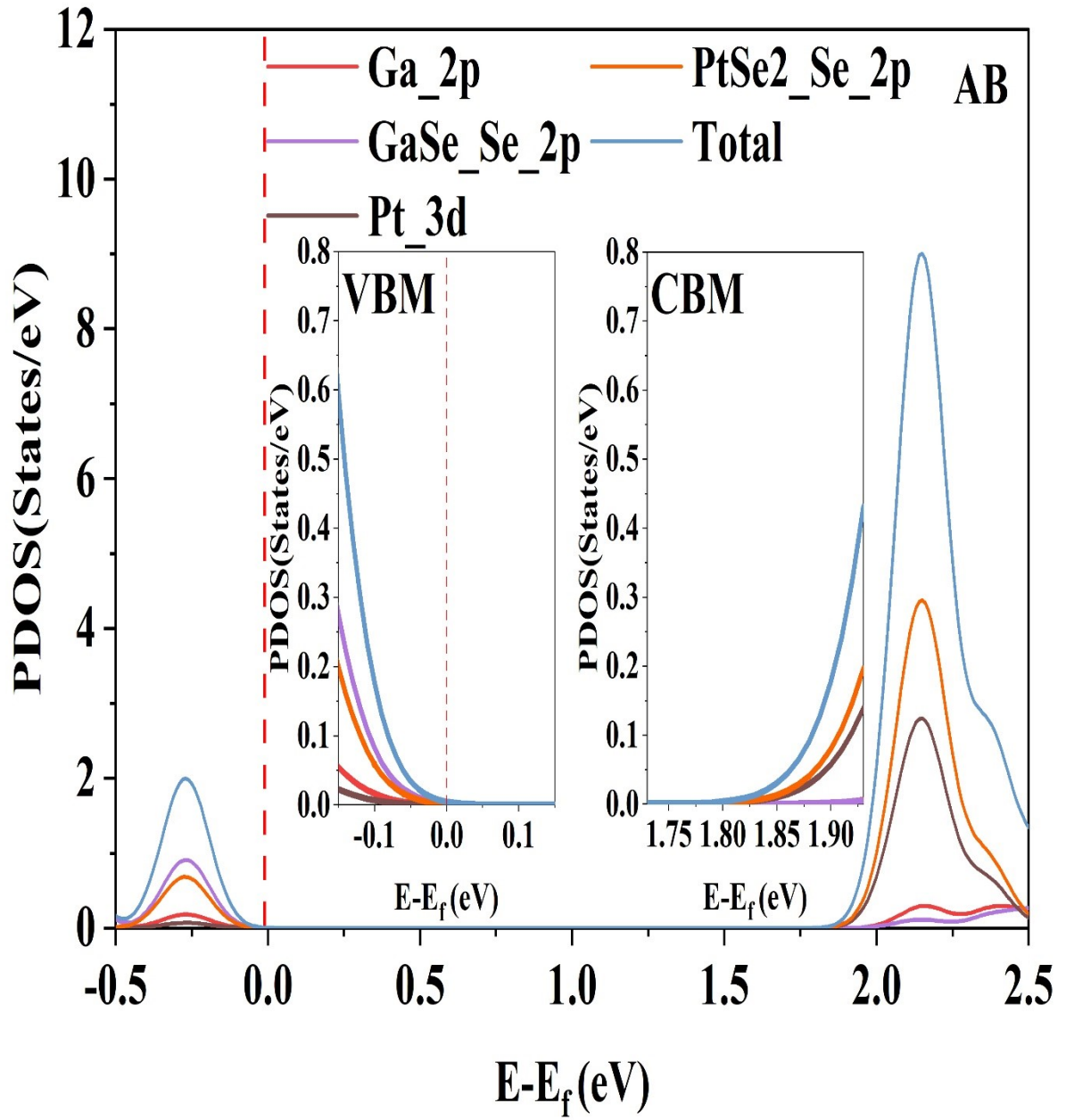
Fig. S2. Enlarged view of VBM and CBM of PDOS of vdwHS-AB
