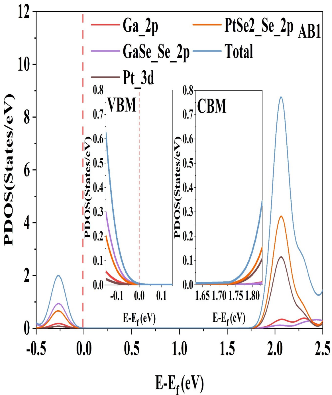
Fig. S3. Enlarged view of VBM and CBM of PDOS of vdWHS-AB1
