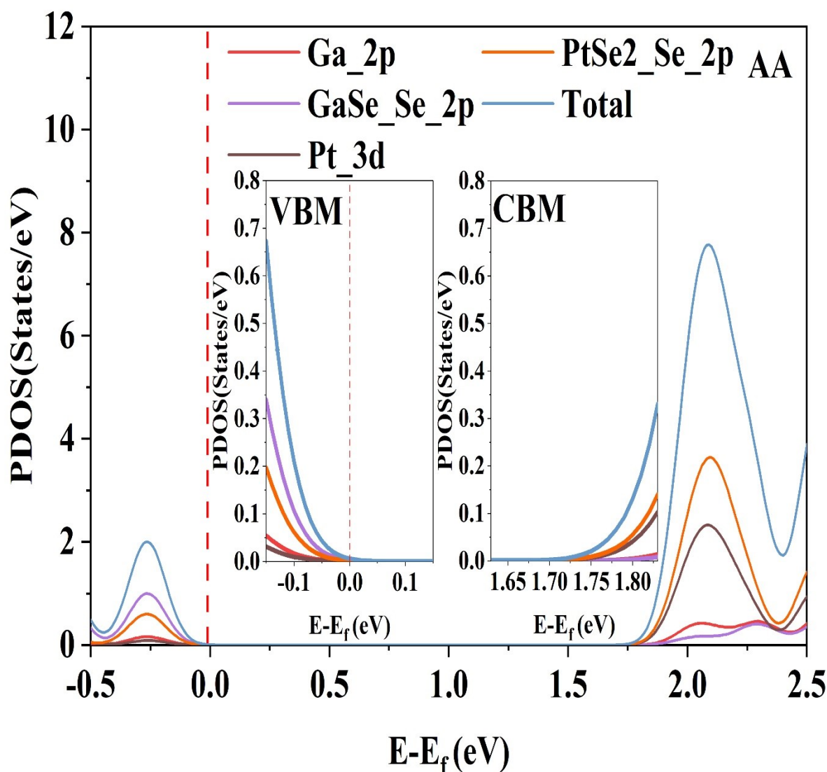
Fig. S1. Enlarged view of VBM and CBM of PDOS of vdWHS-AA
