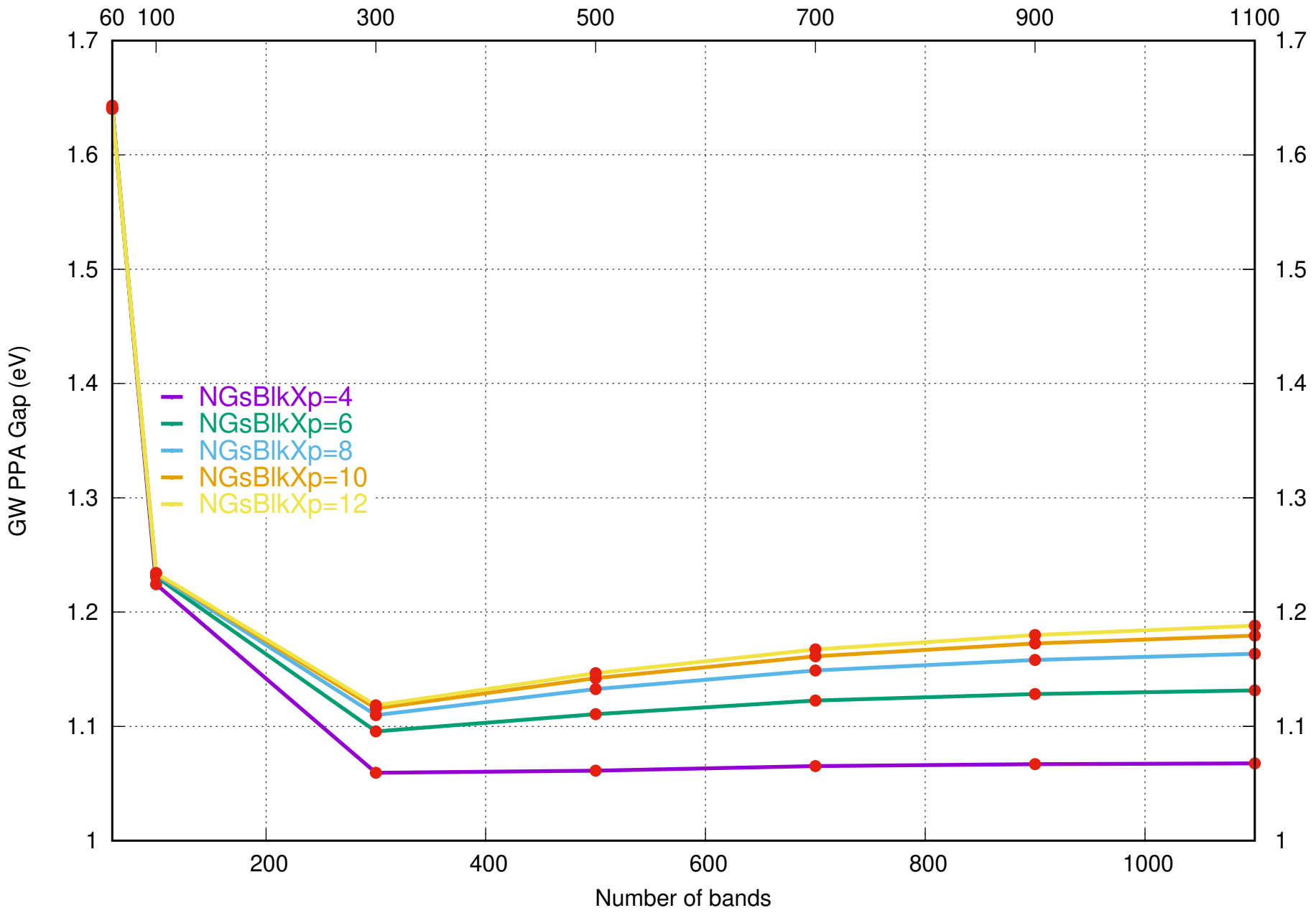
GW PPA gap for (\text{CH}_4)_4\text{NH}_4\text{PbI}_3 with SOC
