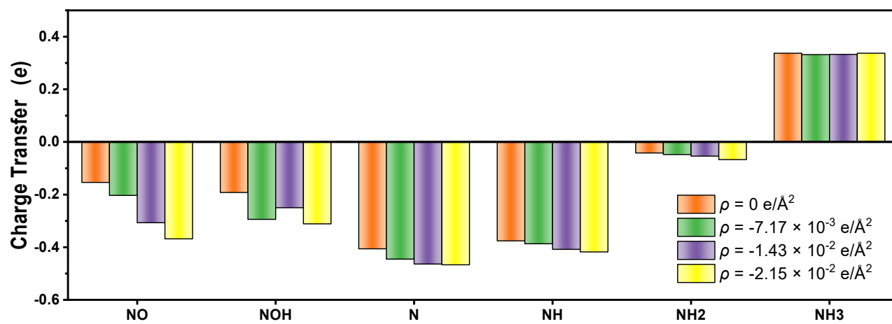
Figure S1. The Mulliken charge analysis.
