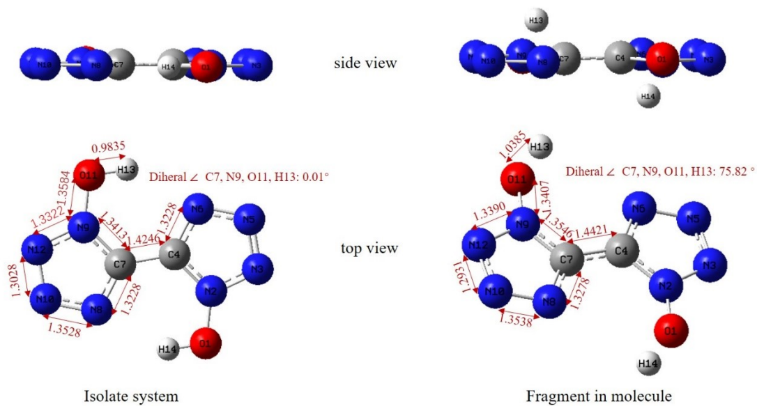
S1: optimized structure comparison of \text{HOC}_2\text{N}_8\text{OH} and fragment \text{C}_2\text{N}_8\text{O}_2\text{H}_2 in molecule II
