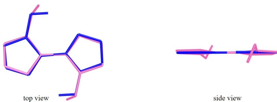
S2: optimized structure of isolate \text{HOC}_2\text{N}_8\text{OH} in blue and mauve fragment \text{C}_2\text{N}_8\text{O}_2\text{H}_2 in molecule II . Total root mean square displacement/deviation (RMSD): 0.3488
