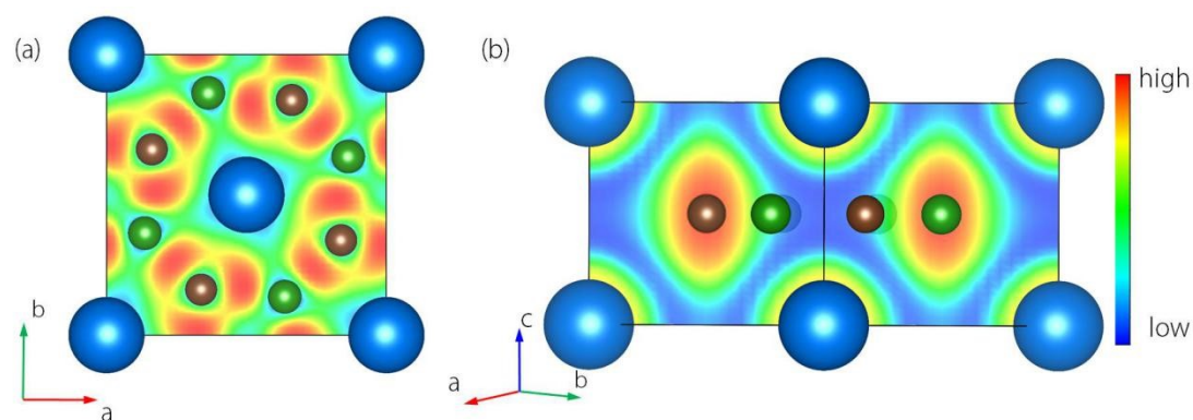
Fig. S1 Different electron localization function planes of \text{YB}_2\text{C}_2 .
