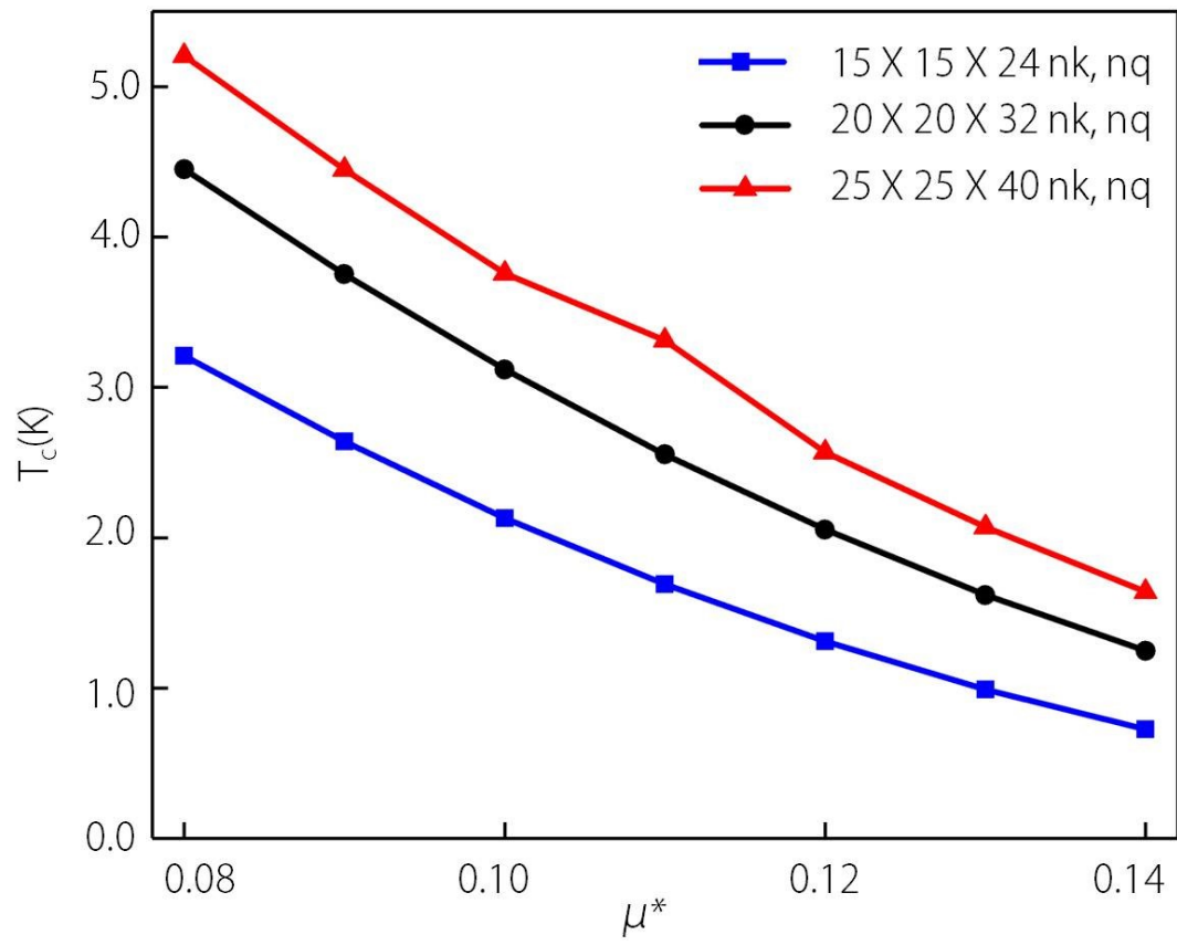
Fig. S2 T_c as a function of Coulomb pseudopotential parameter \mu^* with different k mesh and q mesh interpolated by Wannier functions.
