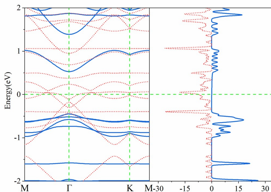
Figure S1 DOS and energy band of Fe-ZN 4 NR obtained by using the HSE06 method.
