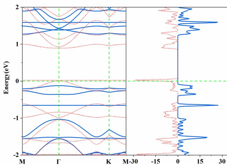
Figure S2 DOS and energy band of Mn-AN 4 NR obtained by using the HSE06 method.
