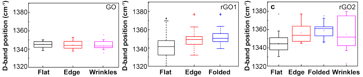
Figure 4: Box plots for D-band peak position in samples of fresh GO, rGO1, and rGO2. The box indicates median, 25th quartile, and 75th quartile for each region, with whiskers indicating minimum to maximum. Outliers are represented with dots. Significant variations are observed for different topographic features in rGO1 and rGO2, where the distributions are relatively consistent in GO. Blue-shifts, in particular at edges and on folded regions, increase with increasing reduction time, from rGO1 to rGO2.
