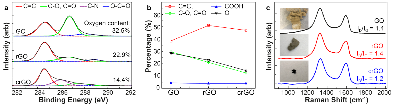
Figure 1: (a) XPS of GO, spontaneously reduced GO (rGO1), and chemically-reduced GO (crGO) with peak fitting of different carbon bonded species. The derived oxygen percentage is labeled for each spectrum. (b) Percentage of sp^2 carbon (red), carboxyl (blue), hydroxyl and carbonyl (green) groups, and total oxygen (black), extracted from the fits in (a) for the three samples. This analysis shows the reduction in oxygen-containing functional groups from the fresh to reduced samples. (c) Micro-Raman spectra and optical images for the GO, rGO, and crGO samples in (a) and (b).
