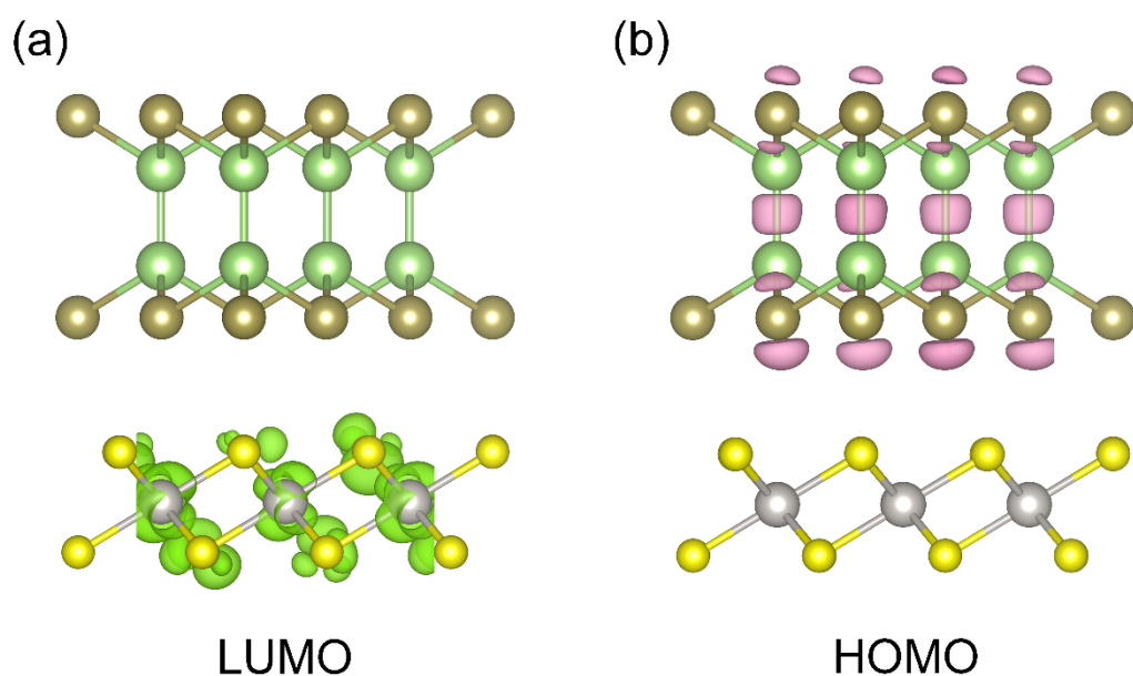
Figure S1 (a) Side view of the LUMO and HOMO of the GaTe/PtS 2 heterojunction, with the isosurface value of 0.005e Å -3 .
