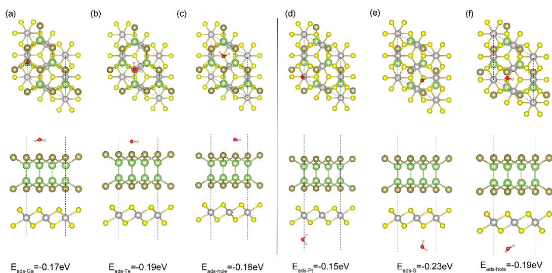
Figure S2 The relaxed structures and adsorption energies of adsorbed H 2 O molecules at different sites on (a)-(c) GaTe surface and (d)-(f) PtS 2 surface, respectively.
