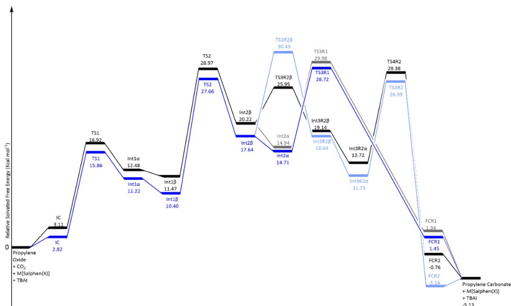
Figure S37 Free energy pathway for the addition of \text{CO}_2 and epoxide with the [\text{InCl}(\text{Salphen})] catalyst. The black line presents the model ligand and the blue the full ligand system with t\text{Bu} groups.
