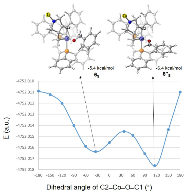
Figure S6. The relaxed potential energy surface scan along the C2-Co-O-C1 dihedral angle.
