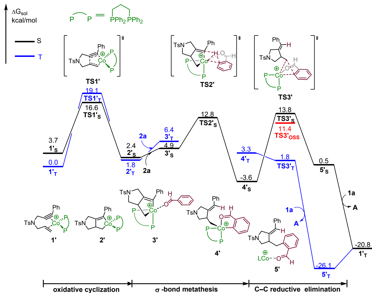
Figure S8. Free energy profiles of the cobalt-catalyzed cyclization of enynes with benzaldehydes forming the hydroarylate product A in the presence of dppp ligand.
