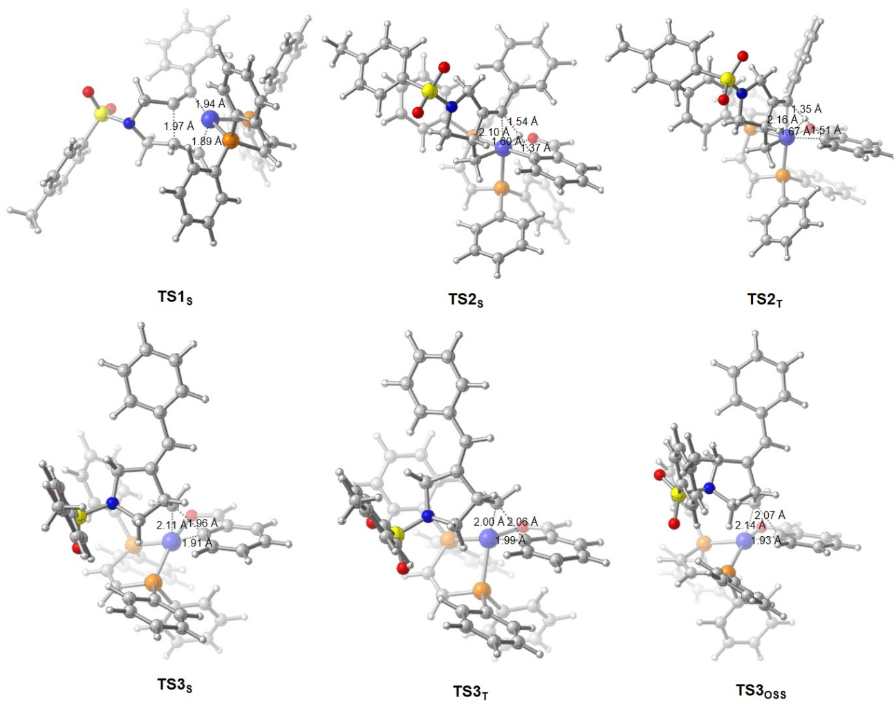
Figure S2. Optimized structures of the key transition states in Figure S1 with selected bond distances.
