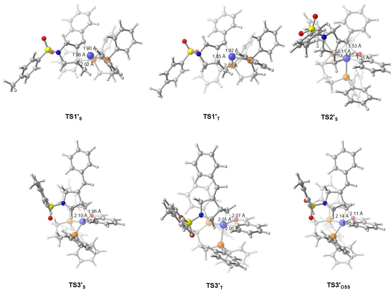
Figure S9. Optimized structures of the key transition states in Figure S8 with selected bond distances.
