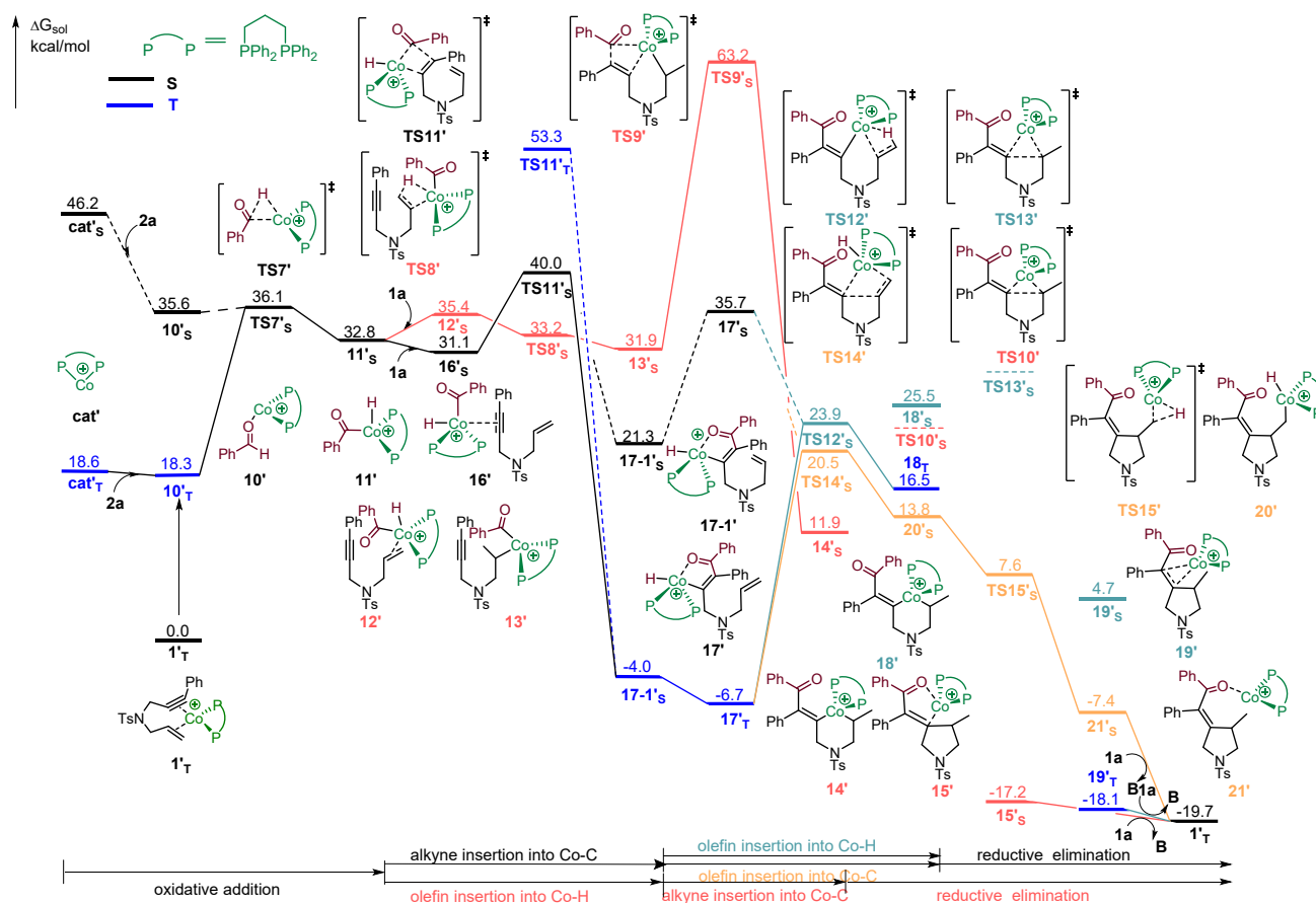
Figure S12. Free energy profiles of the other possible catalytic cycles for the formation of product B in the presence of dppp ligand.
