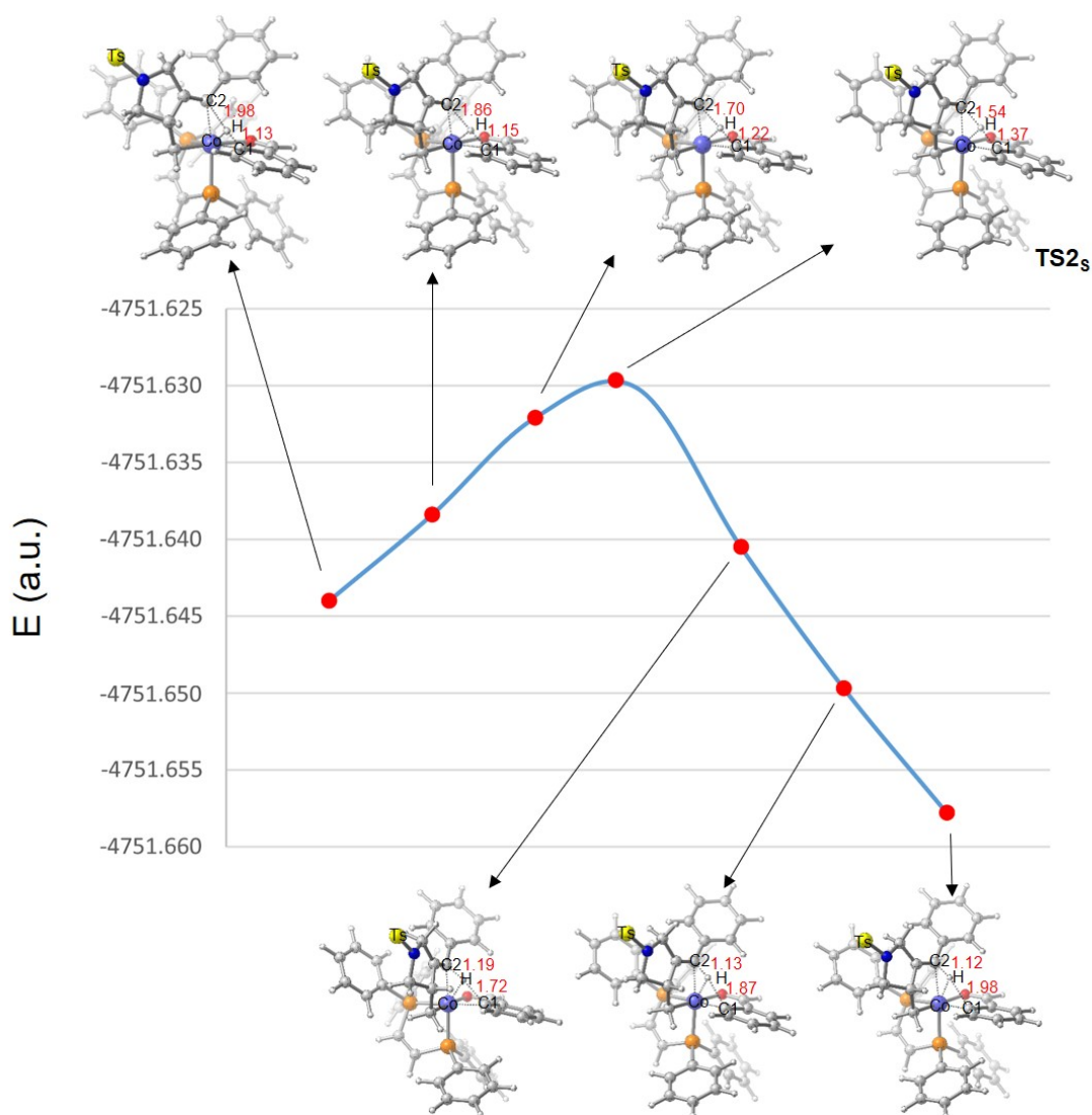
Figure S5. The geometry changes along the intrinsic reaction coordinate (IRC) of TS2_s , with selected bond distances in Å.
