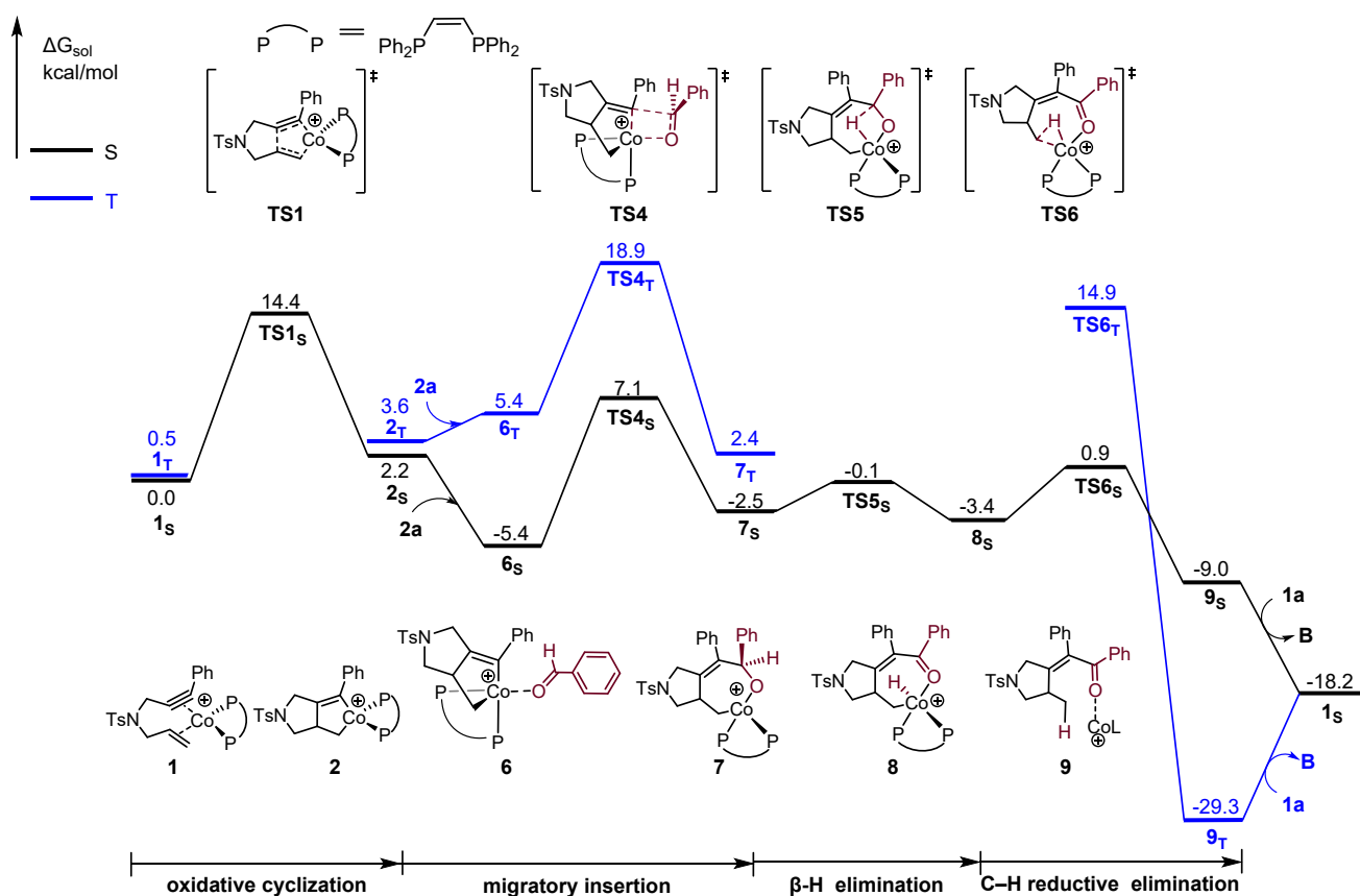
Figure S3. Free energy profiles of the cobalt-catalyzed cyclization of enynes with benzaldehydes forming the hydroacylative product B in the presence of dppen ligand.
