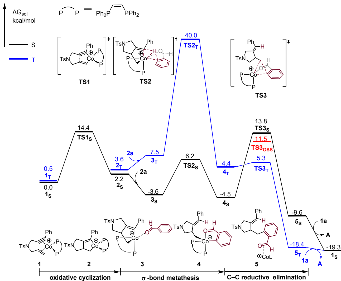
Figure S1. Free energy profiles of the cobalt-catalyzed cyclization of enynes with benzaldehydes forming the hydroarylate product A in the presence of dppen ligand.
