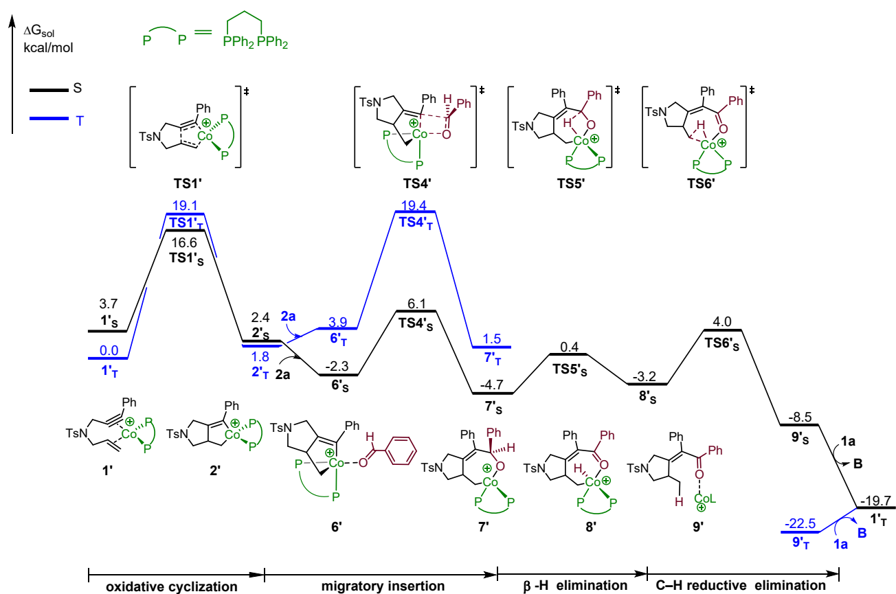
Figure S10. Free energy profiles of the cobalt-catalyzed cyclization of enynes with benzaldehydes forming the hydroacylative product B in the presence of dppp ligand.
