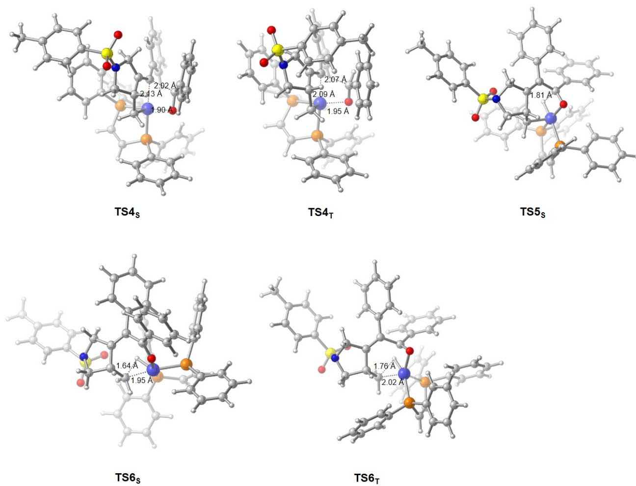
Figure S4. Optimized structures of the key transition states in Figure S3 with selected bond distances.
