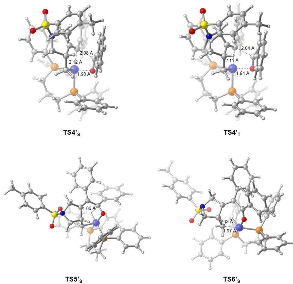
Figure S11. Optimized structures of the key transition states in Figure S10 with selected bond distances.
