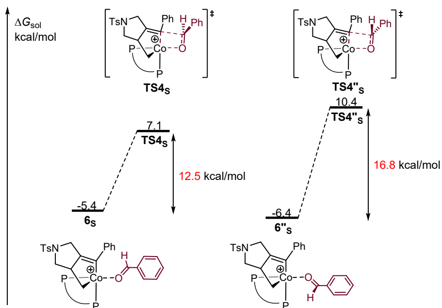
Figure S7. A comparison of the migratory insertion step from 6 s or 6'' s intermediate.
