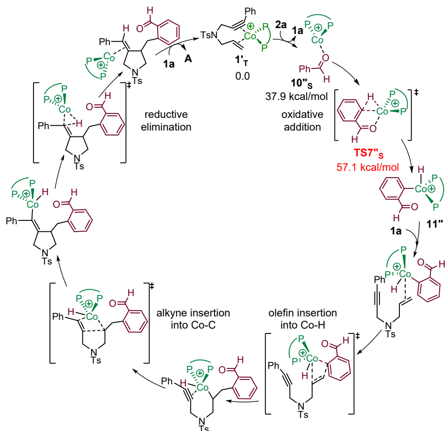
Figure S14. The other possible reaction pathway for formation of product A in the presence of dppp.
