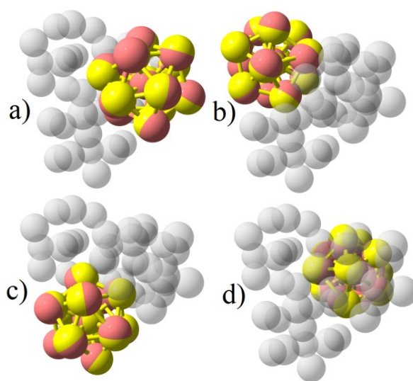
Figure S1. Separated Au 13 units (yellow) embedded in the Au 48 core (grey), in comparison to an idealized I h -Au 13 structure (pink). For details see main manuscript.
