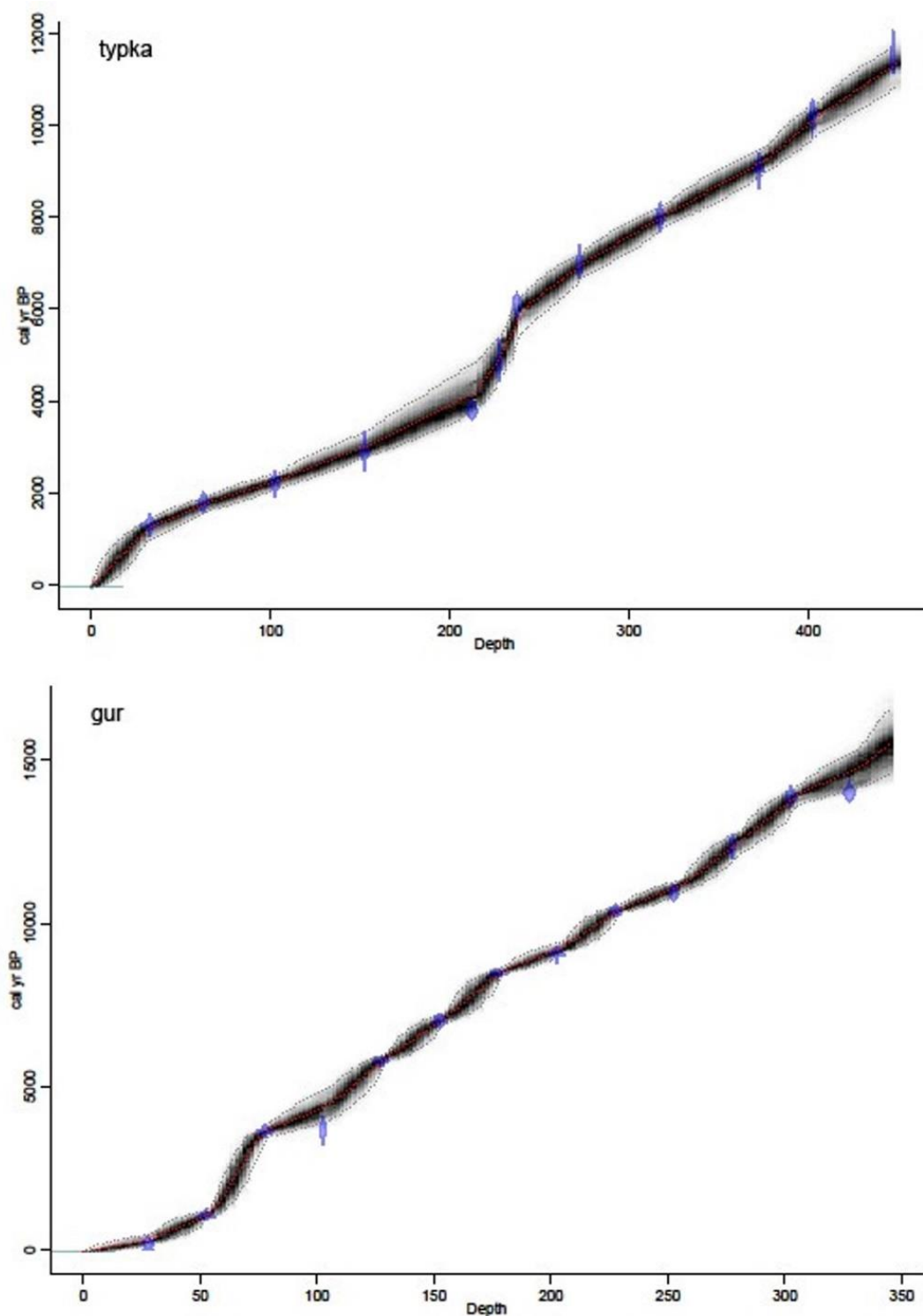
Supplementary Fig. 2 Radiocarbon dates ( ^{14}\text{C} yr BP) calibrated with Bacon's method (Blaauw and Christen, 2011) to calendar years before present (cal yr BP) vs. peat depth for the Tyapka and Gur peat cores.
