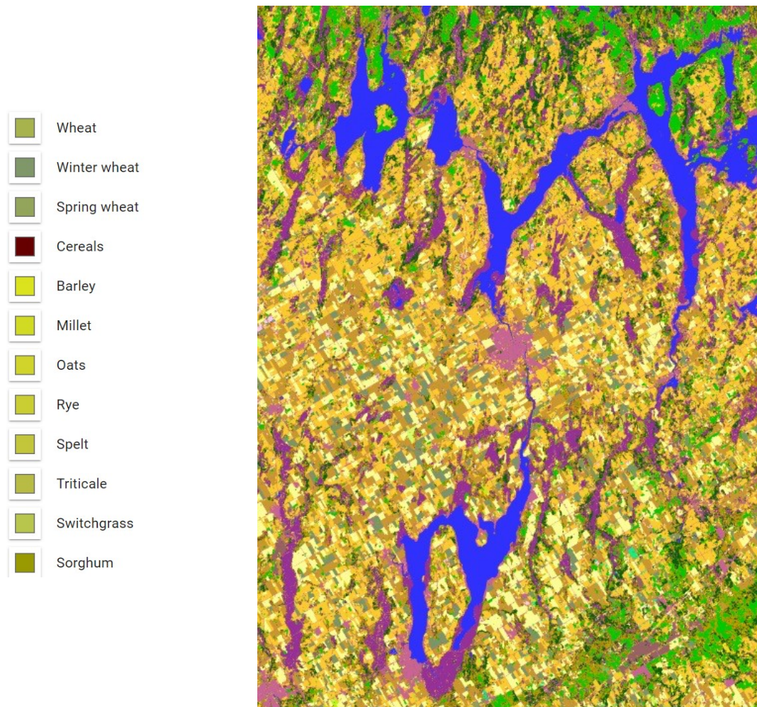
Figure S1: Land cover map delineated based on agricultural land use across the sampled watersheds. Data obtained from GovCan's 2022 Annual Crop Inventory ( https://open.canada.ca/data/en/dataset/ba2645d5-4458-414d-b196-6303ac06c1c9 ).
