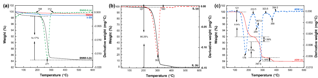
Figure S1. (a) TG (solid line) and DTG (dashed line) curves of pristine h-BN, BNNS, BNNS-IL, (b) TG (solid line) and DTG (dashed line) of pure IL, (c) TG (solid line) and DTG (dashed line) of pure ADM.
