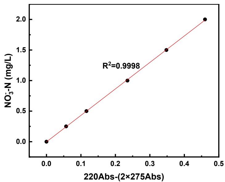
Fig.S1. UV-Vis spectrophotometer NO 3 - -N standard curve
