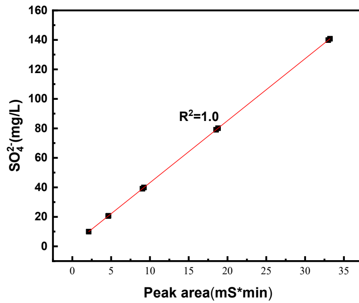
Fig.S4.Ion chromatograph SO 4 2- standard curve
