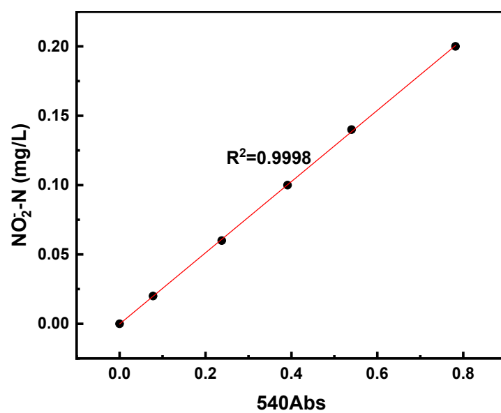
Fig.S2. UV-Vis spectrophotometer NO 2 - -N standard curve
