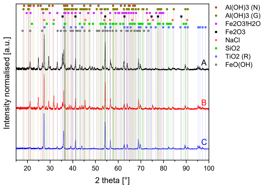
Figure S2. XRD spectra of sludge samples A, B and C from wastewater.
