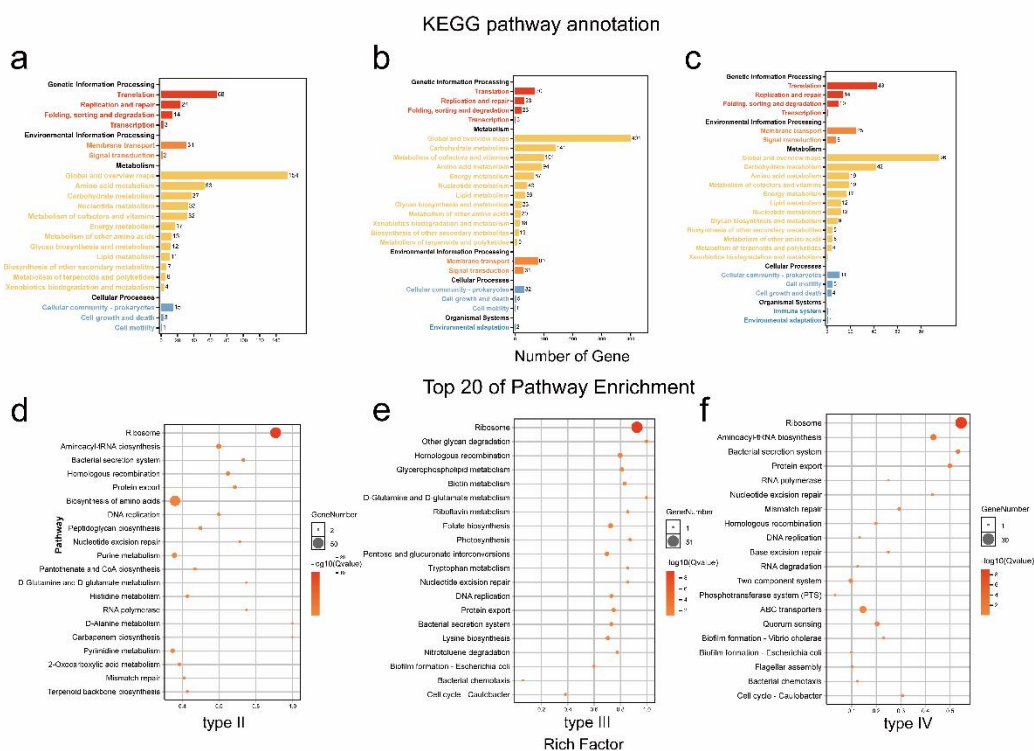
a, b, c Bar chart of enrichment pathway classification statistics of three types of RS. d, e, f Significant enrichment bubble plots of three types of RS.
