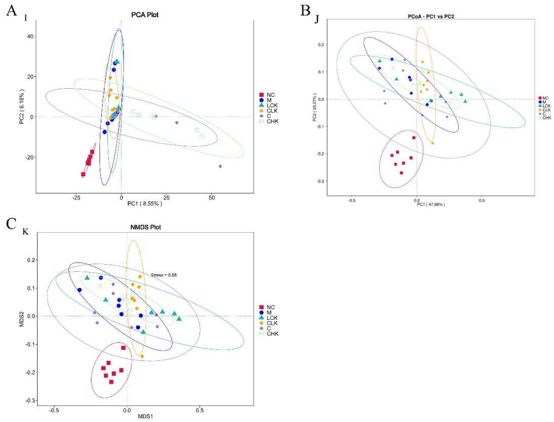
Figure S3 \beta -diversity analyzed by PCA (A), PCoA (B), NMDS (C).
