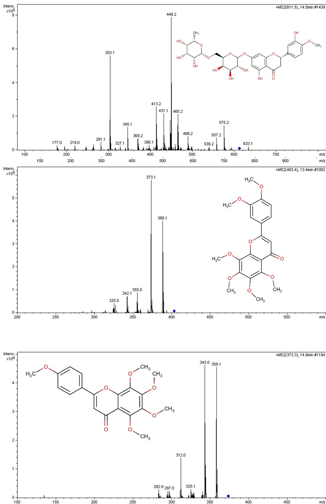
S1. The mass spectra of hesperidin, nobiletin and tangeretin.
