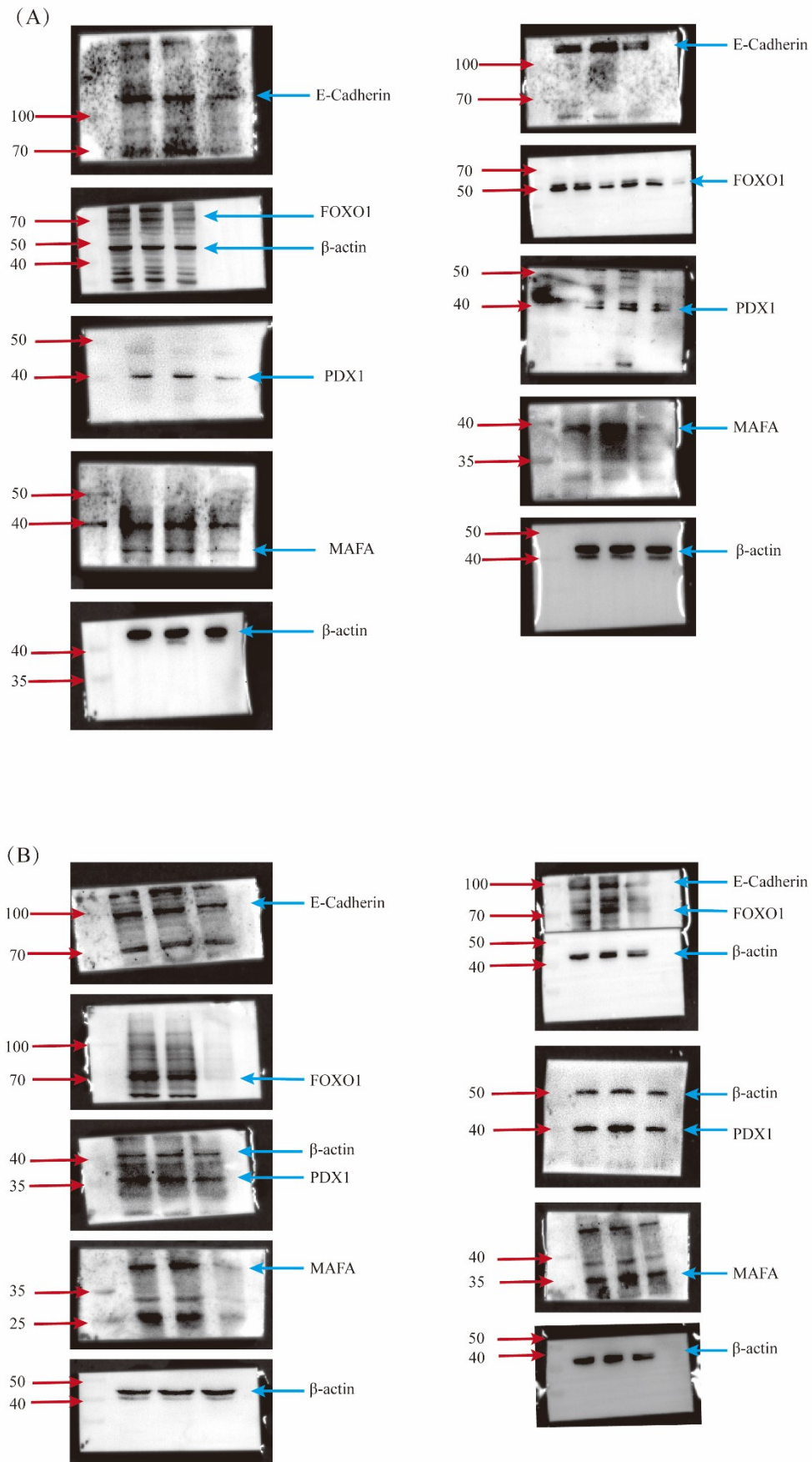
Fig. 8. Change of related factors in Rin-m5f cells and Min6 cells via gene silencing of FOXO1.
