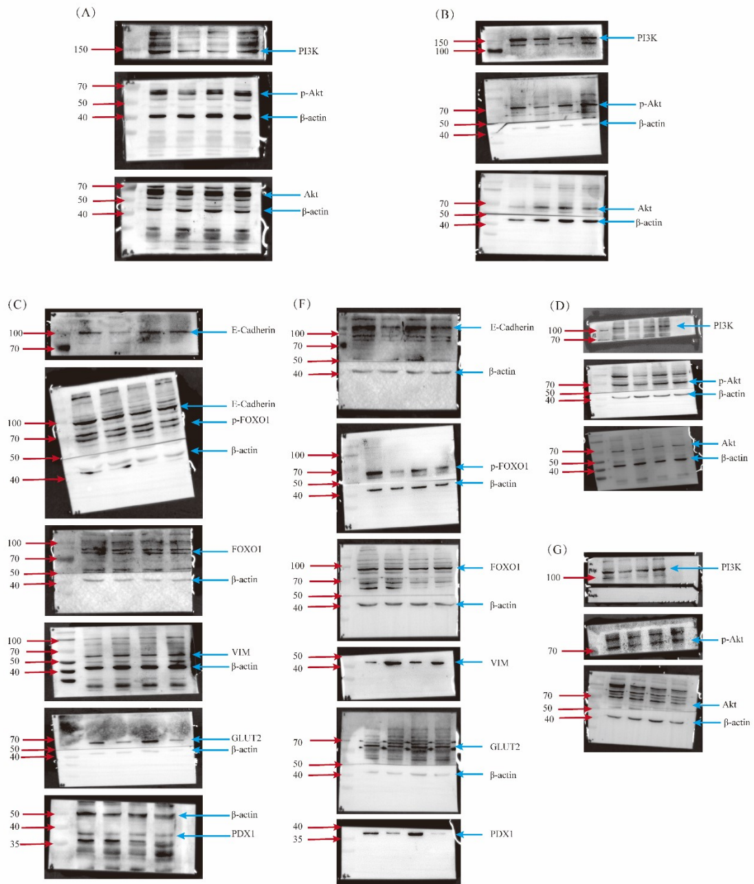
Fig. 7. Signaling pathway activated by LGP9 treatment.
