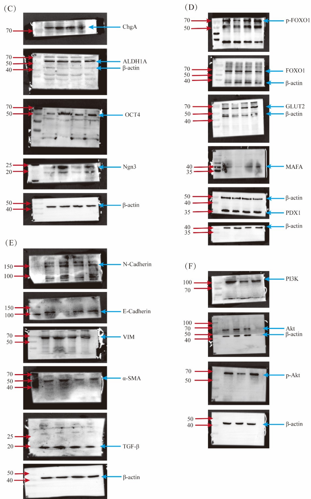
Fig. 4. The effect of LGP9 on the pancreas of HFD-STZ-induced T2D mice.
