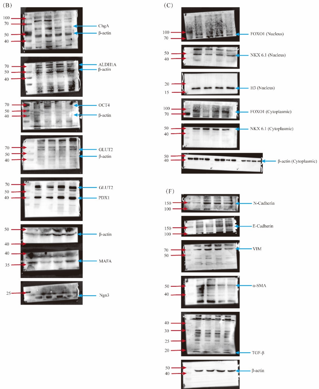
Fig. 5. The effect of LGP9 on \beta -cell dedifferentiation of IIG-treated Rin-m5f cells.
