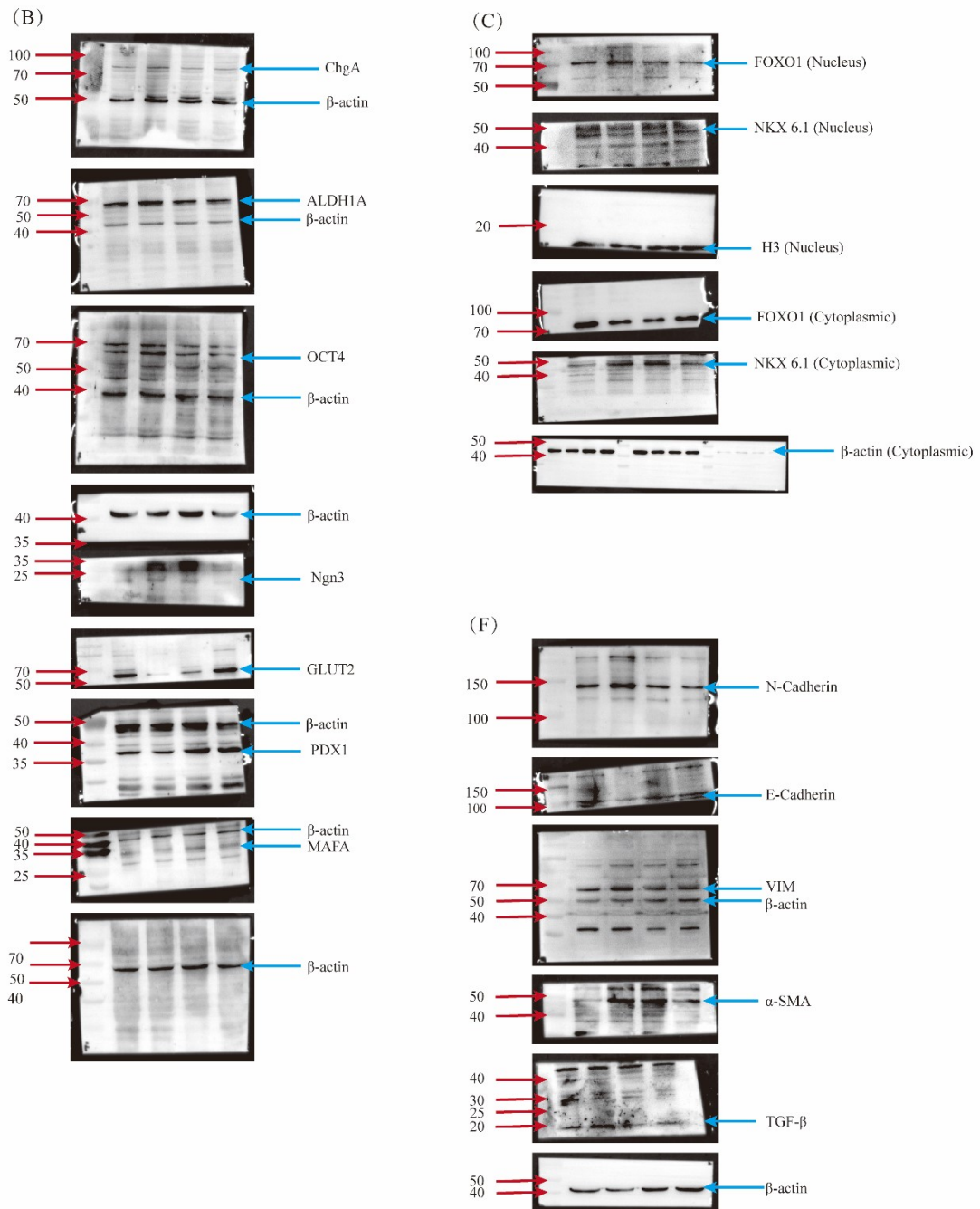
Fig. 6. The effect of LGP9 on \beta -cell differentiation of HG/PA-treated Min6 cells.
