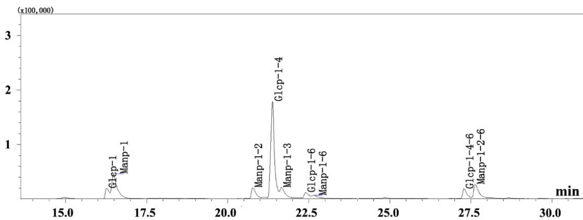
Figure S1. Total ion chromatograph (TIC) of partial methylated alditol acetates (PMAA) fragmentation of the derivatives from LPE-2.
