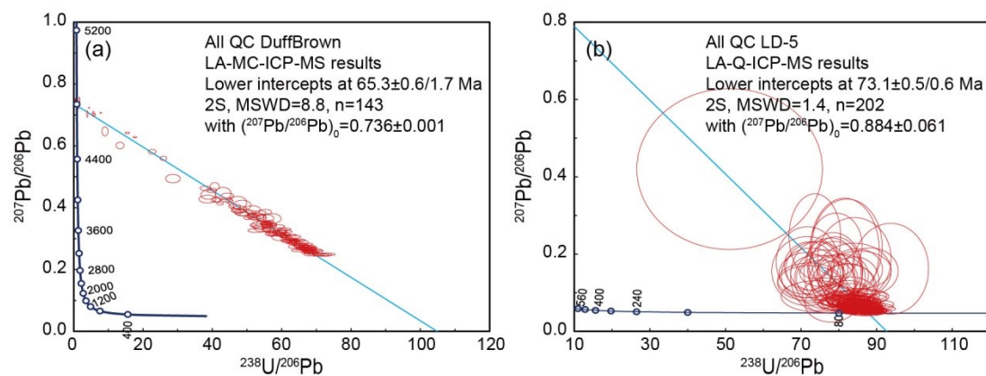
Figure S1. T-W diagram of (a) DuffBrown and (b) LD-5 quality control standards. Ellipses are 2S errors.
