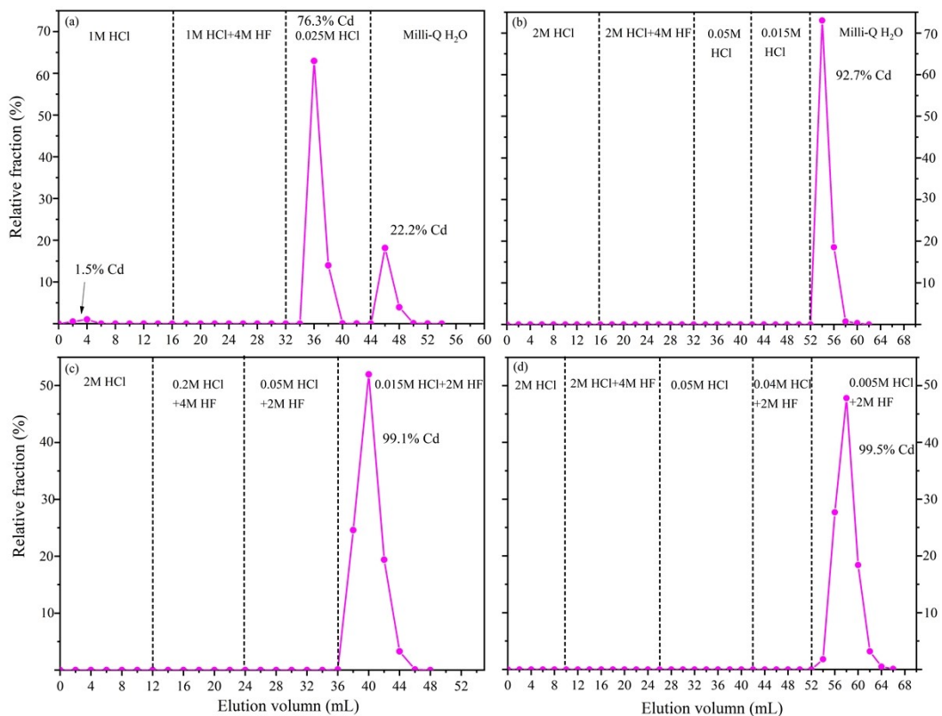
Fig. S1. Elution curves of Cd purification procedures using different reagents. Corresponding to Fig. 1a-1d, only Cd and its recovery rate at each step is included.
